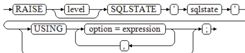
Figure 11-36 raise_sqlstate::=
