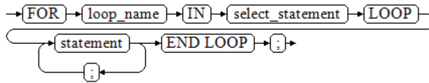
Figure 11-33 FOR_AS_loop::=
