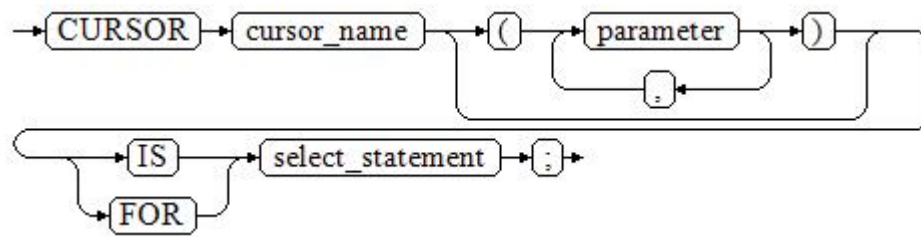
Figure 11-26 static_cursor_define::=
