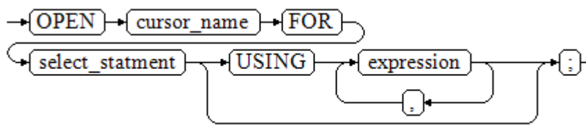
Figure 11-30 open_dynamic_cursor::=
