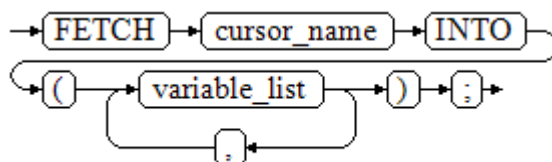
Figure 11-31 fetch_cursor::=
