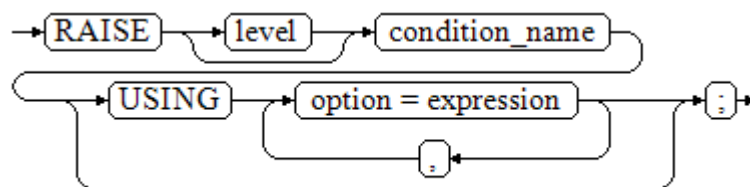
Figure 11-35 raise_condition::=
