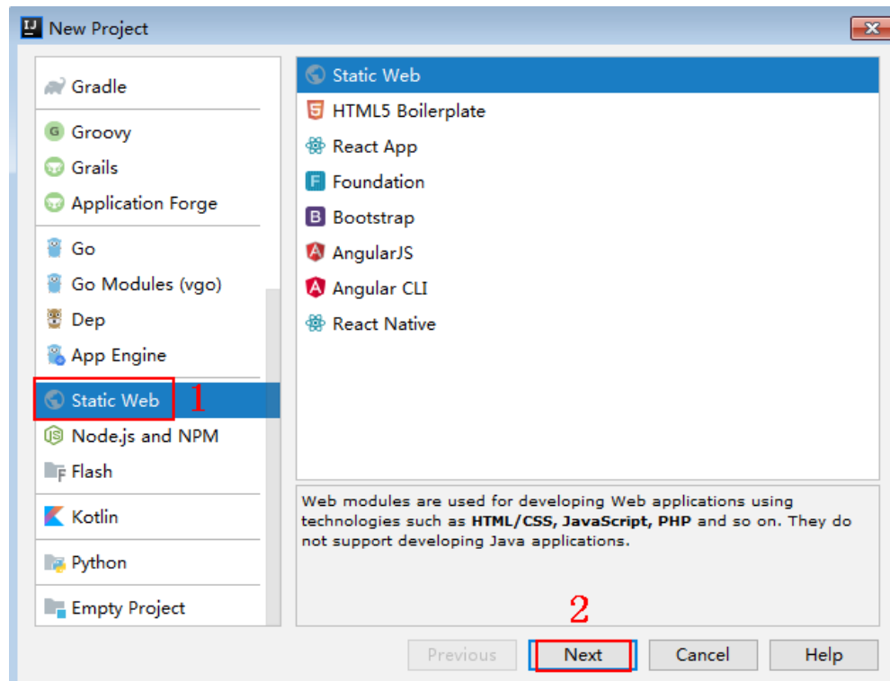
Figure 2-22 Static Web
