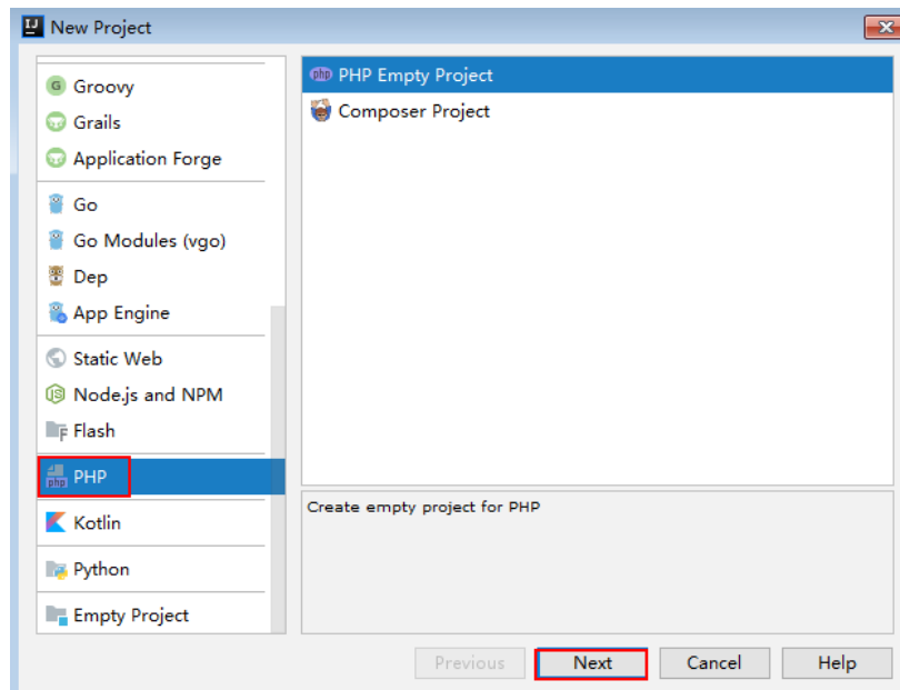
Figure 2-30 PHP
