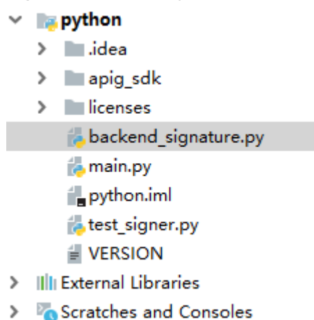
Figure 6-7 Directory structure
