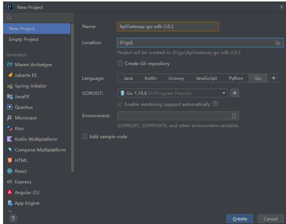
Figure 2-15 Go
