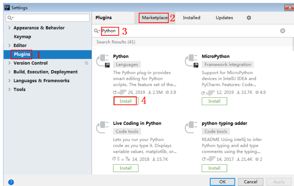
Figure 2-17 Installing the Python plug-in
