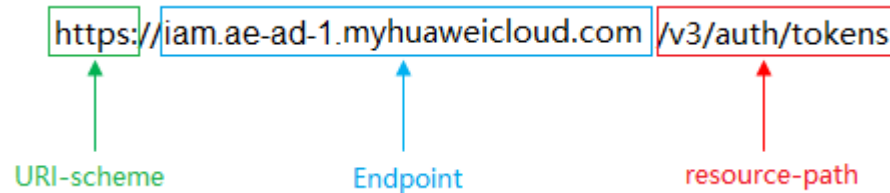
Figure 2-1 Example URI
