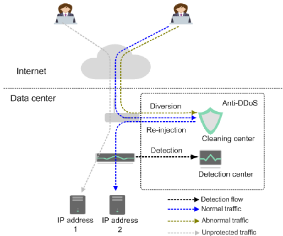
Figure 2-4 Network topology
