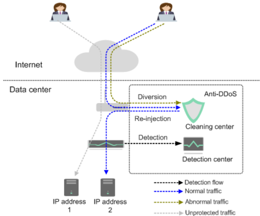
Figure 2-4 Network topology
