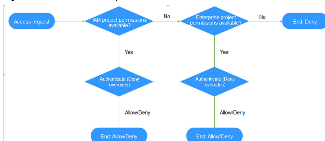
Figure 2-17 Authentication process
