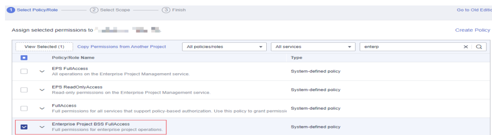
Figure 2-12 Selecting permissions
