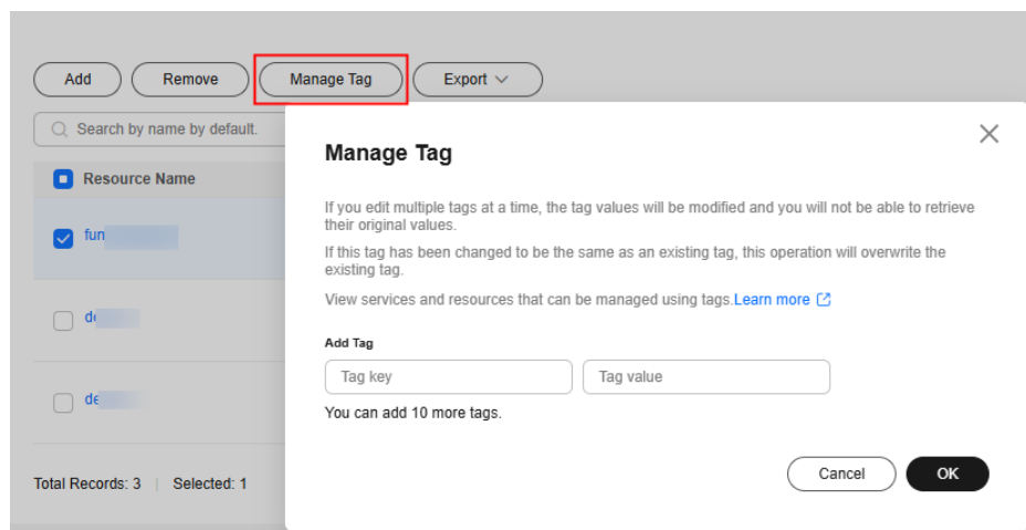
Figure 2-15 Managing tags
