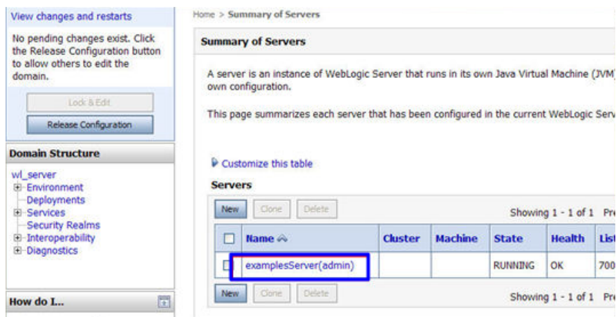
Figure 3-12 Target server
