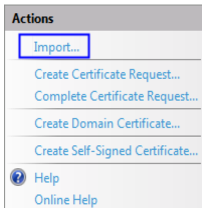
Figure 3-7 Import
