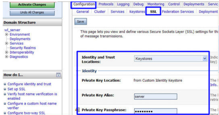
Figure 3-17 Private key
