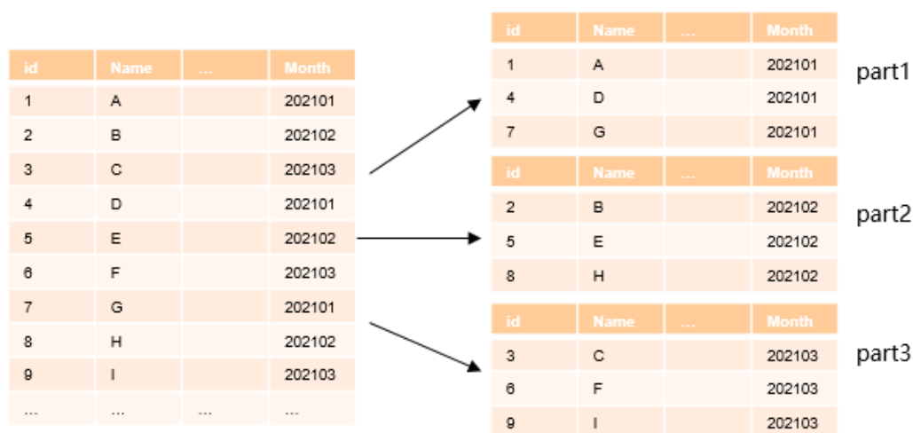
Figure 5-1 Example of a partitioned table
