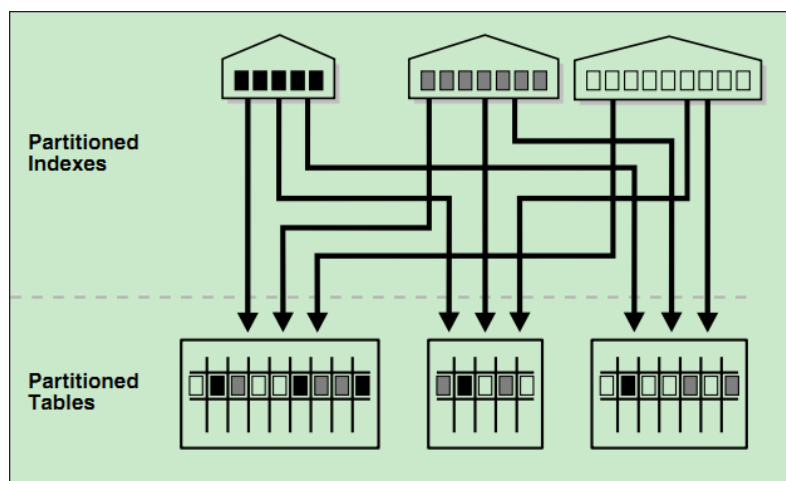
Figure 5-4 Global partitioned index
