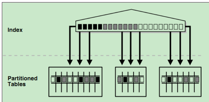
Figure 5-3 Global non-partitioned index
