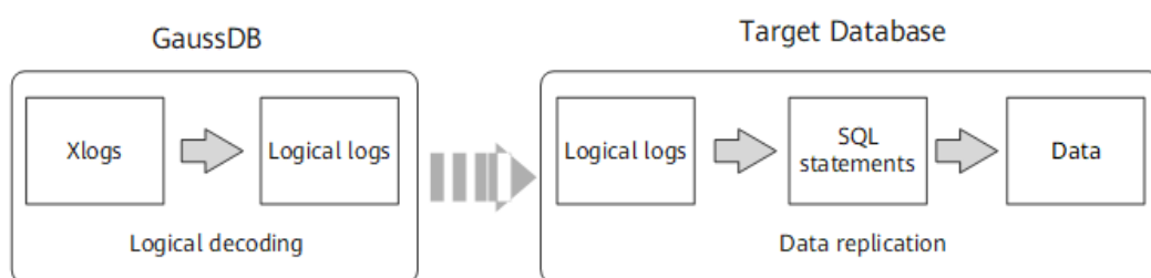
Figure 4-1 Logical Replication
