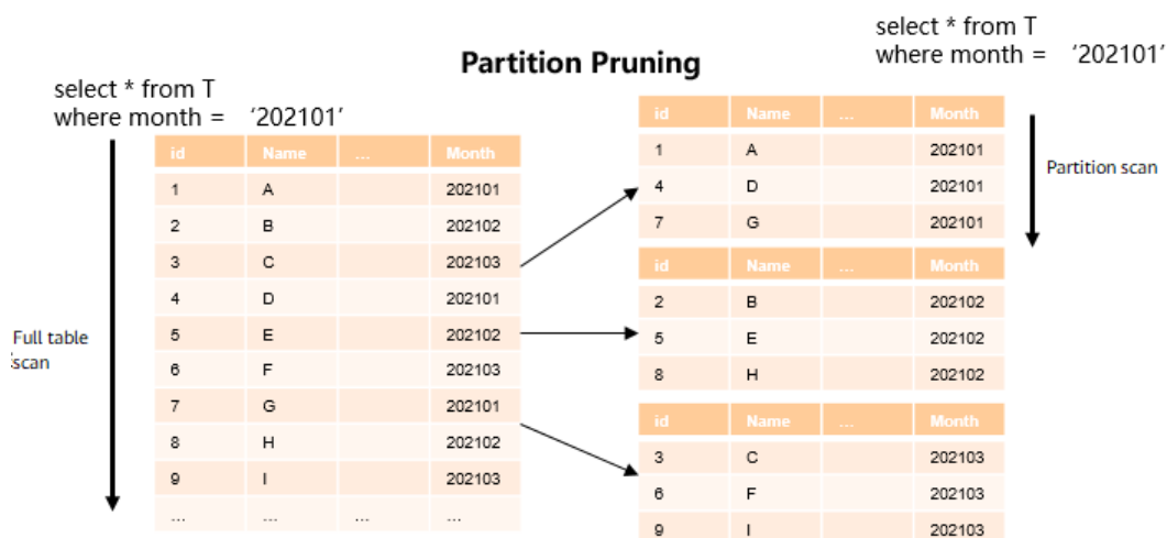
Figure 5-2 Example of partition pruning
