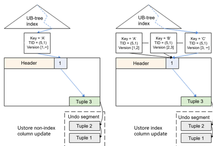
Figure 6-1 UB-tree processing during data updates
