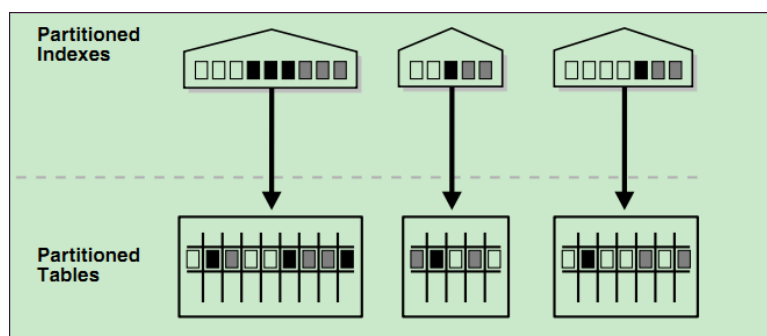
Figure 5-5 Local partitioned index
