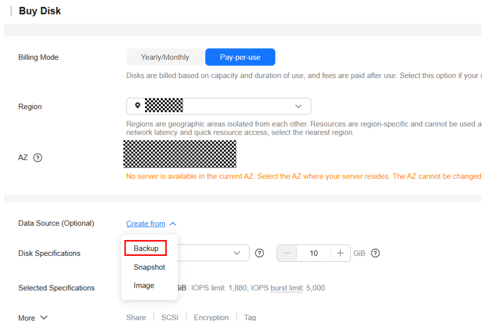
Figure 2-2 Create from backup
