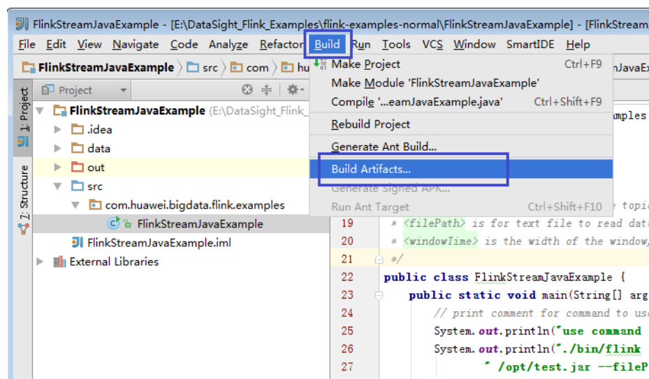
Figure 10-41 Building Artifacts
