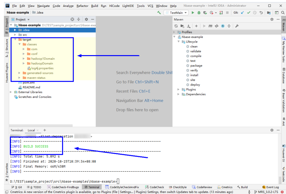
Figure 11-20 Compilation completed
