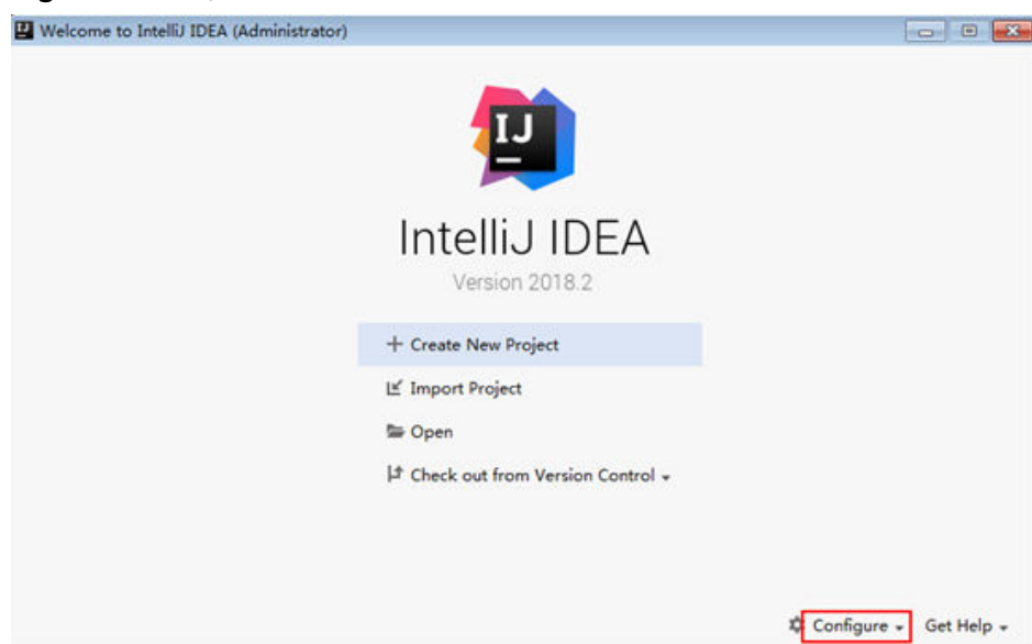
Figure 13-3 Quick Start
