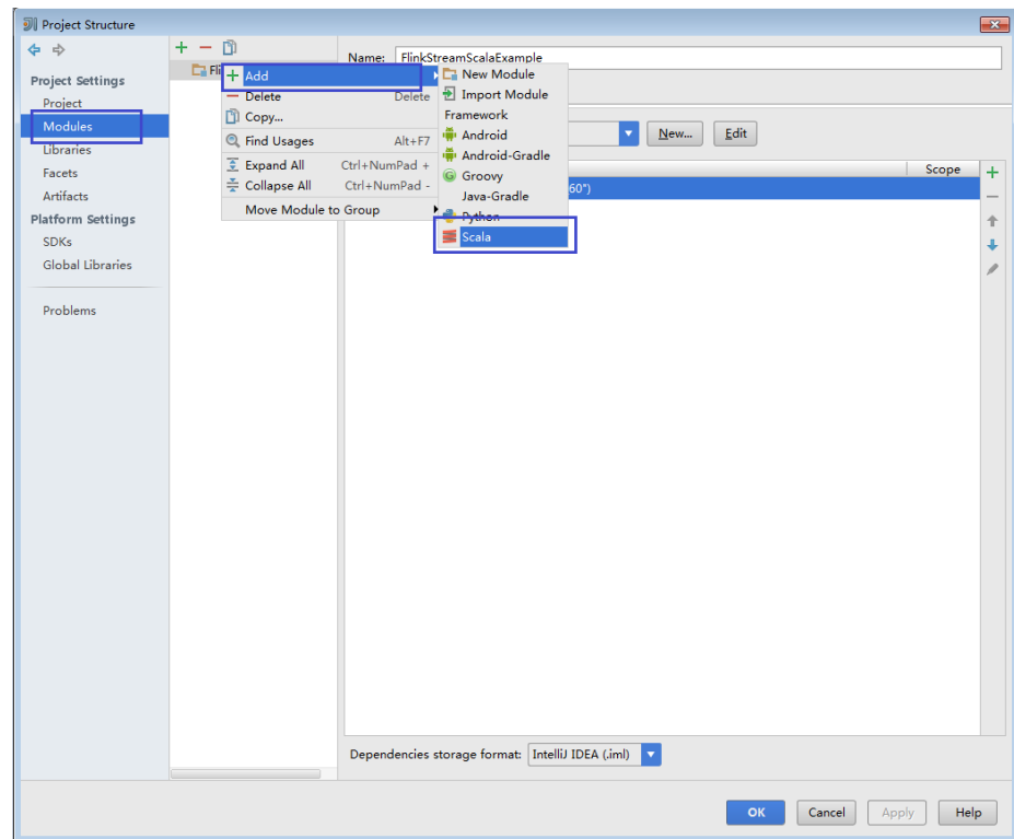
Figure 10-23 Selecting Scala
