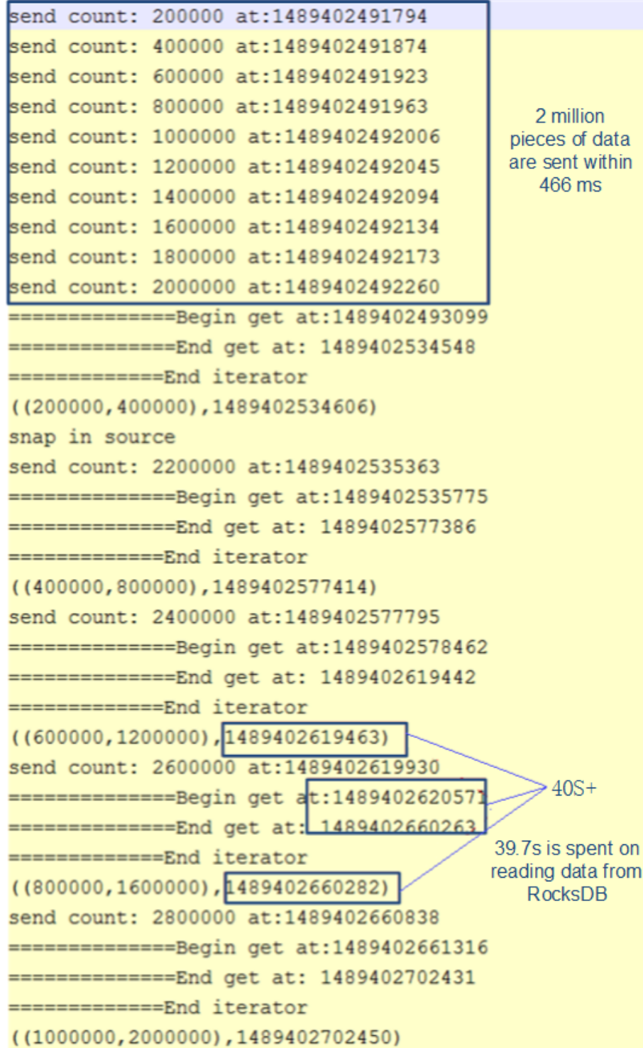
Figure 10-63 Time monitoring
