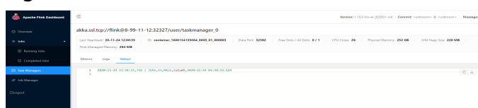
Figure 10-54 Execution result
