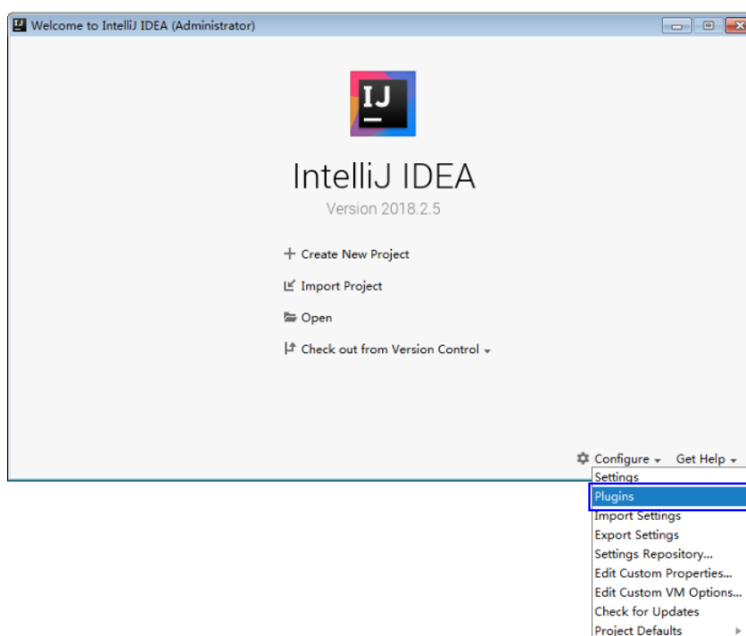
Figure 27-16 Plugins
