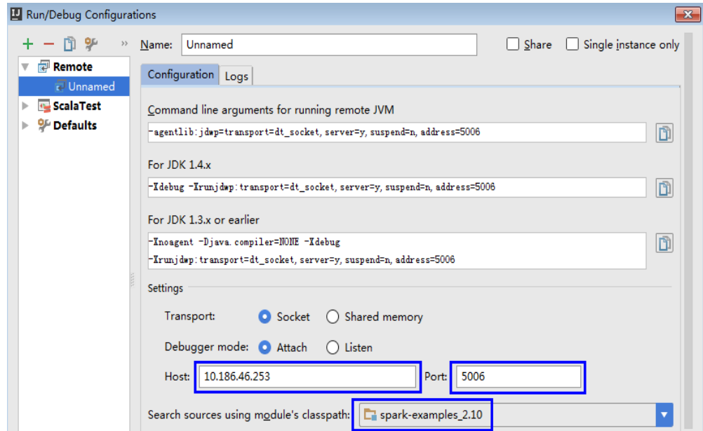
Figure 28-46 Choosing Remote
