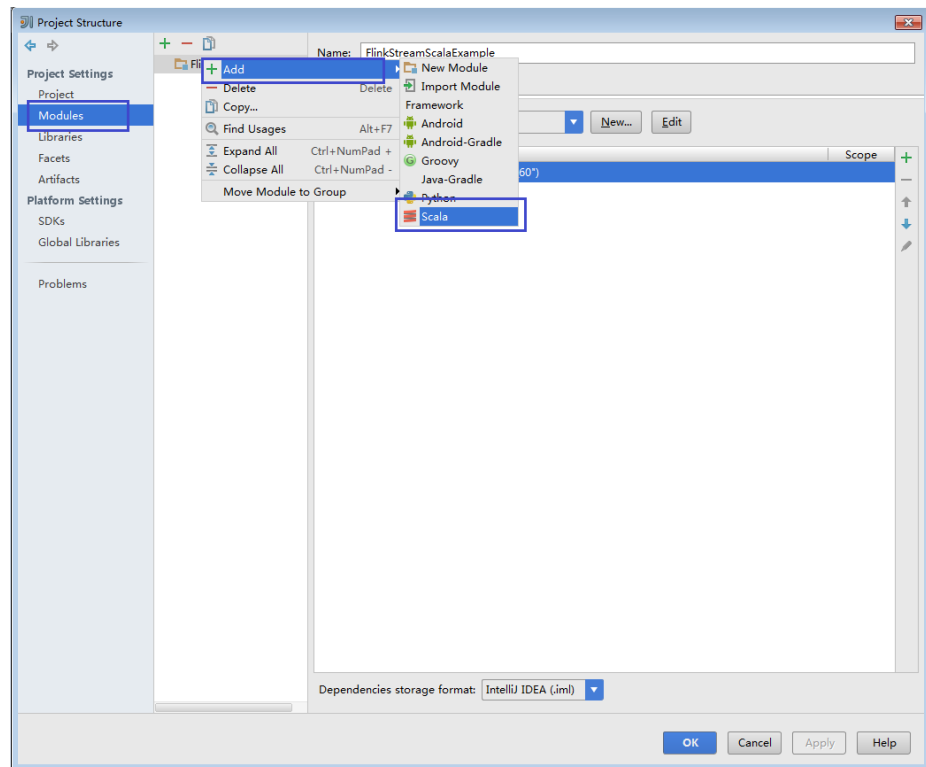
Figure 9-22 Selecting Scala
