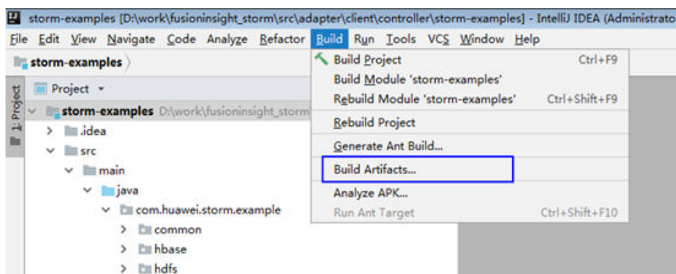
Figure 30-17 Build Artifacts
