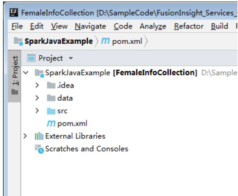
Figure 28-24 Imported projects
