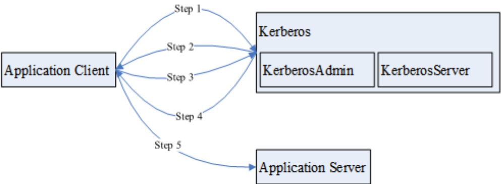
Figure 6-1 Kerberos architecture
