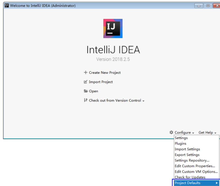
Figure 27-11 Configure
