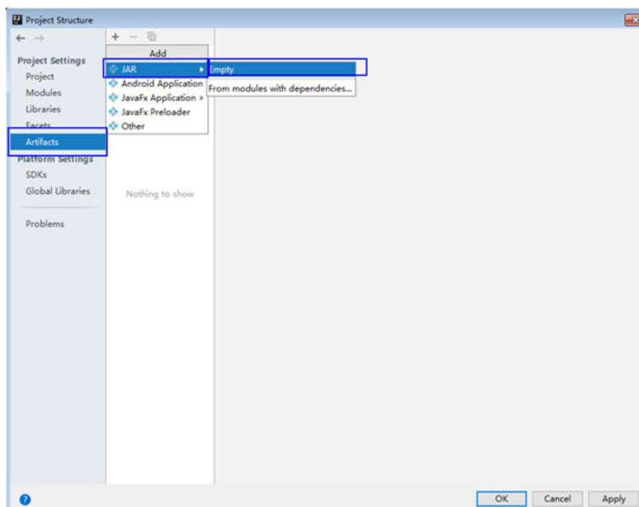
Figure 19-13 Adding Artifacts
