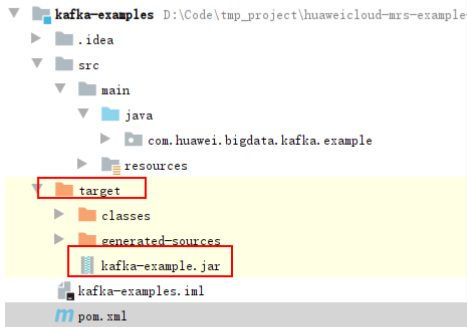
Figure 19-18 File location
