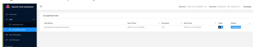
Figure 9-56 completed job
