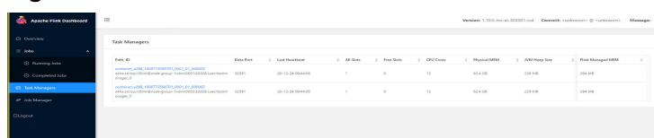
Figure 10-56 Submitted task
