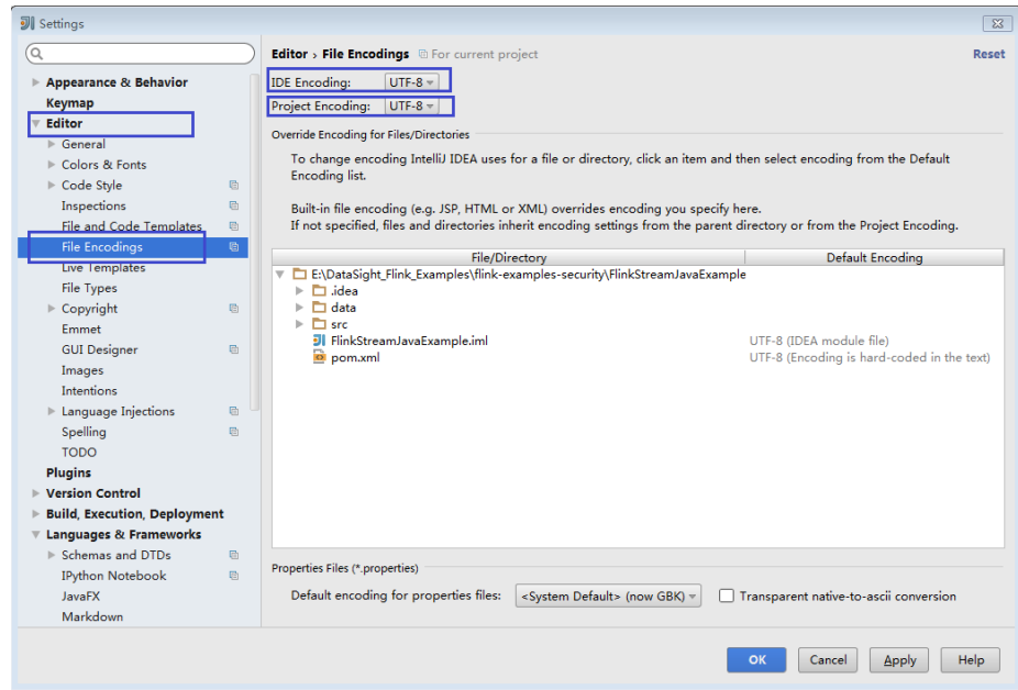
Figure 9-29 Settings
