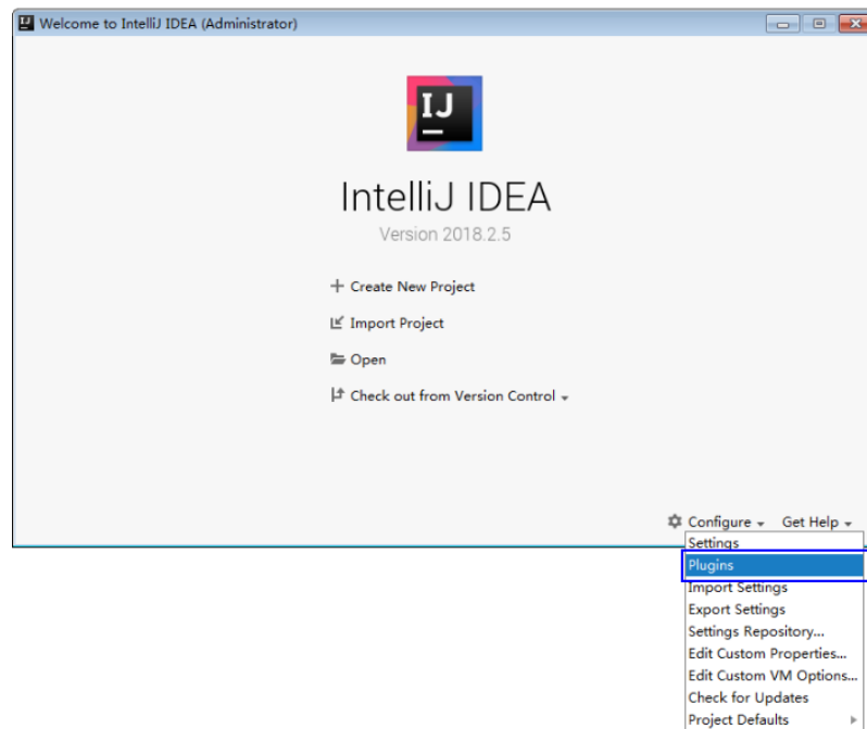
Figure 28-16 Plugins
