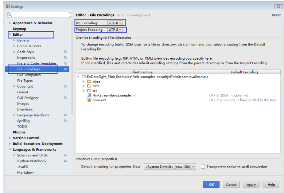
Figure 10-30 Settings
