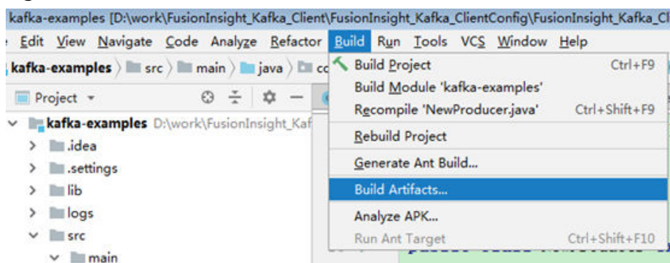
Figure 19-16 Build Artifacts
