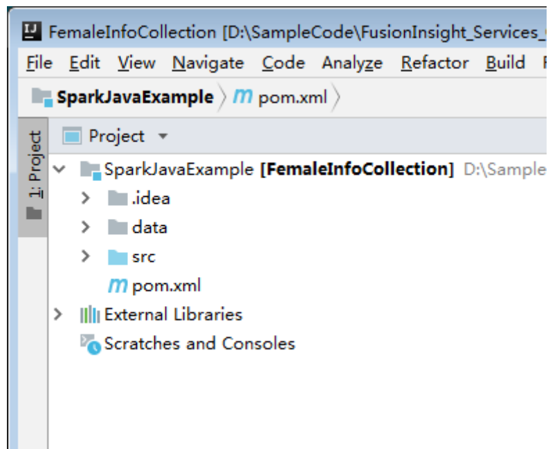
Figure 27-24 Imported projects
