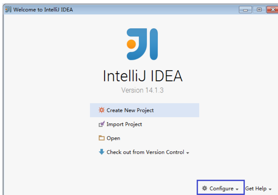
Figure 9-5 Choosing Configure
