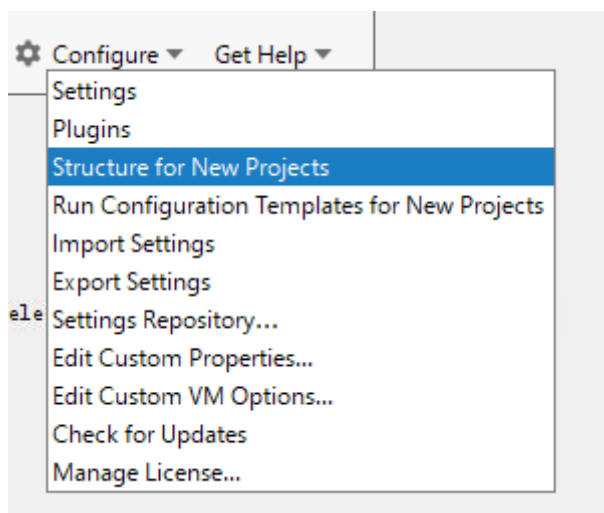
Figure 11-3 Configure
