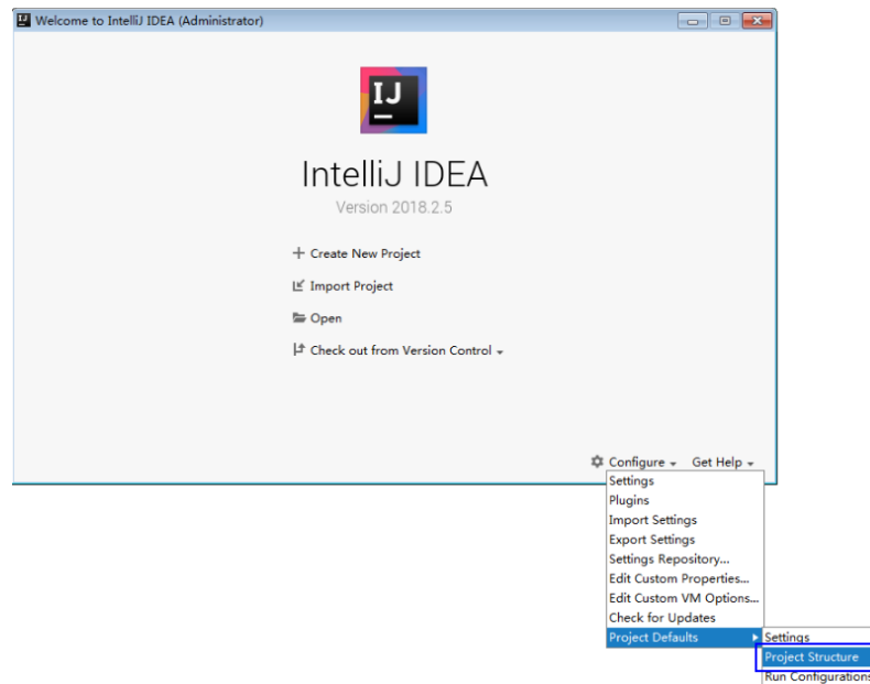
Figure 28-12 Project Defaults
