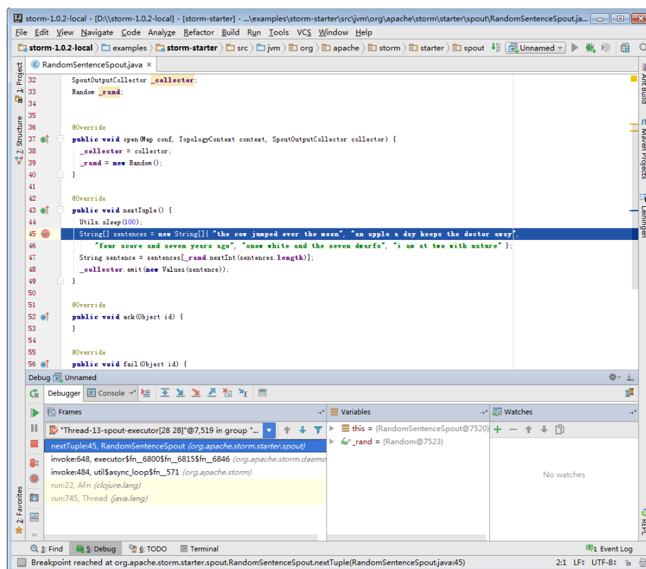
Figure 29-25 Debugging
