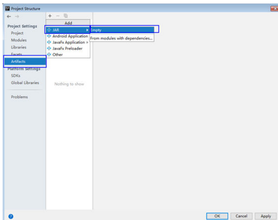
Figure 29-14 Adding Artifacts
