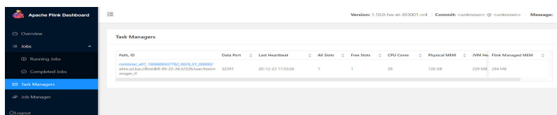
Figure 9-54 submitted task
