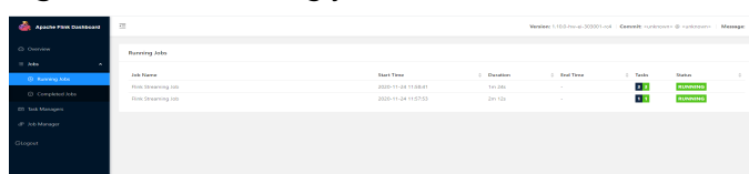
Figure 10-52 Running jobs
