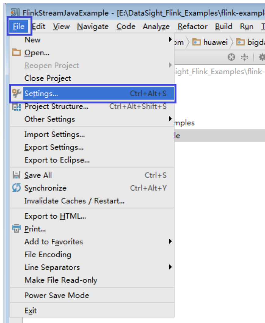
Figure 9-28 Choosing Settings
