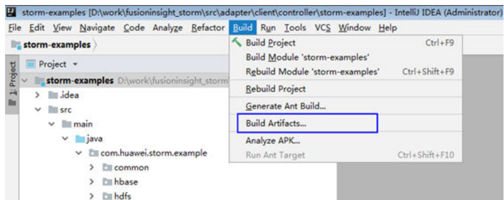
Figure 29-17 Build Artifacts
