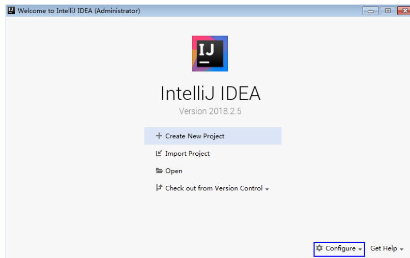
Figure 28-10 Quick Start
