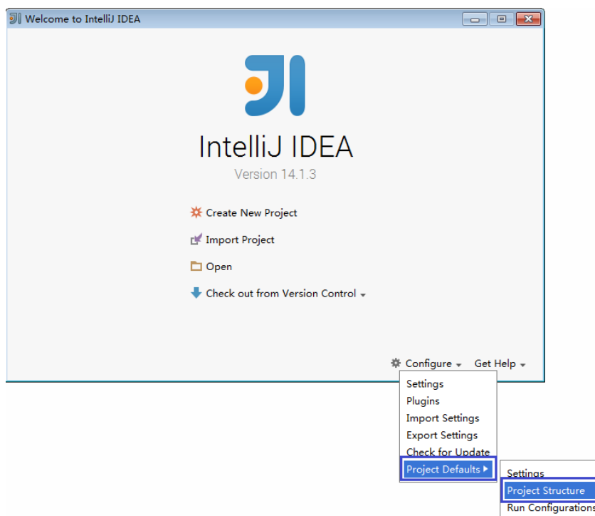
Figure 9-7 Project Defaults
