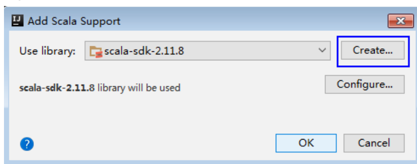
Figure 28-27 Create...
