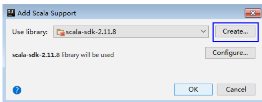
Figure 27-27 Create...
