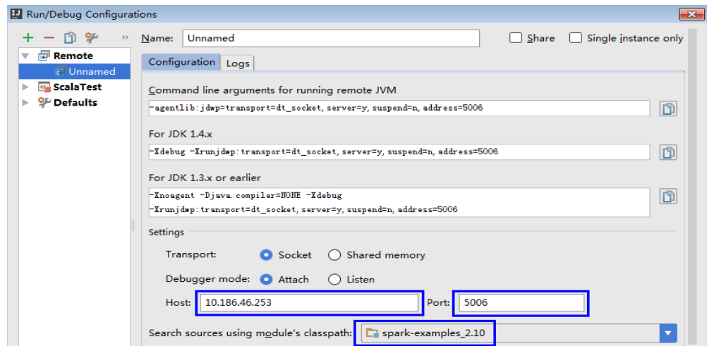
Figure 27-47 Configuring parameters
