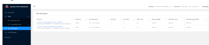
Figure 10-53 Submitted task
