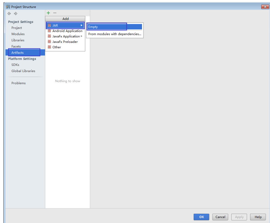
Figure 10-38 Adding Artifacts
