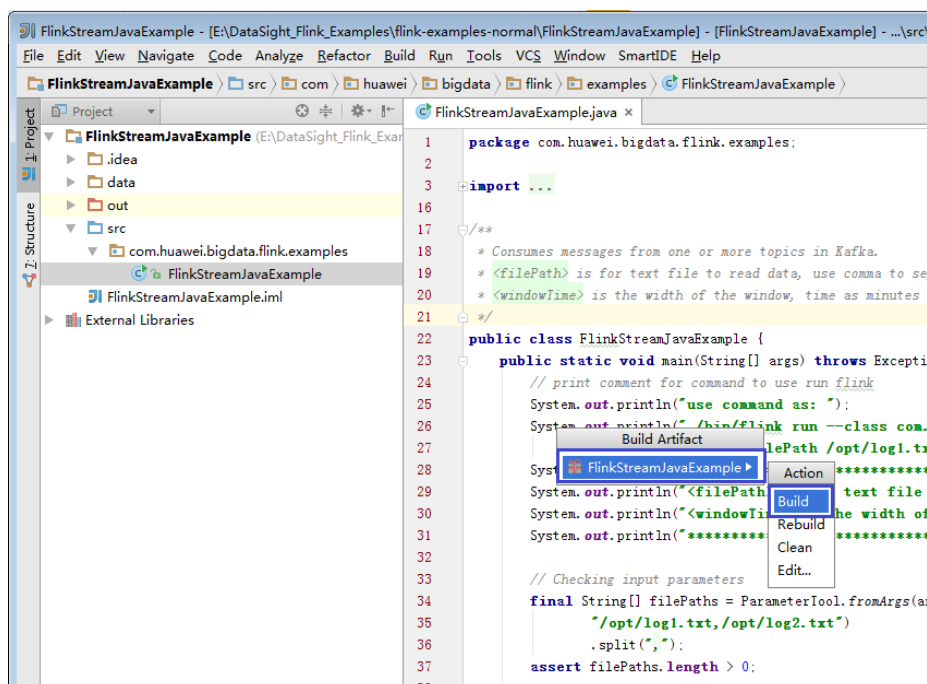
Figure 10-42 Build
