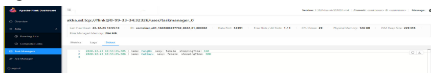
Figure 9-58 execution result
