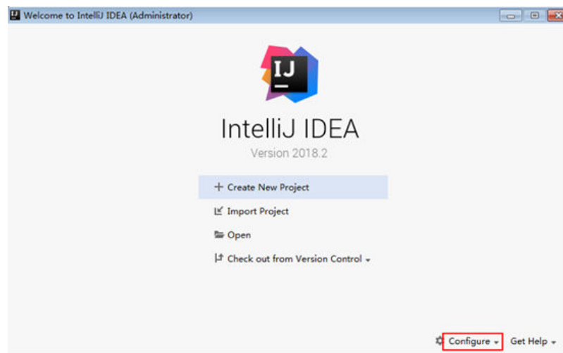
Figure 19-2 Quick Start
