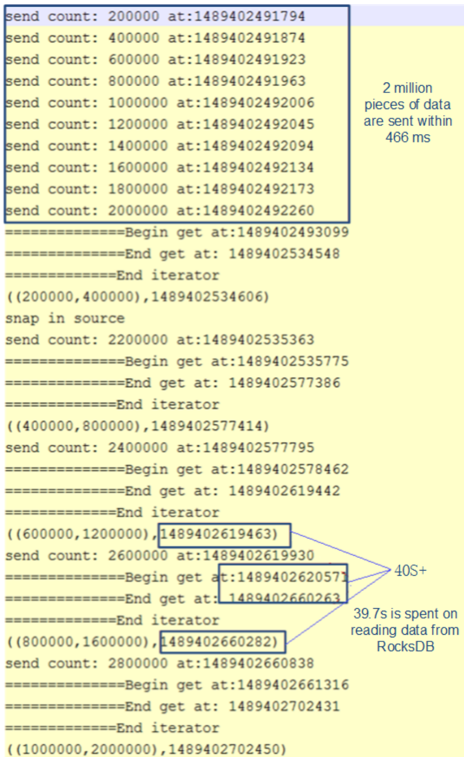
Figure 9-70 Time monitoring
