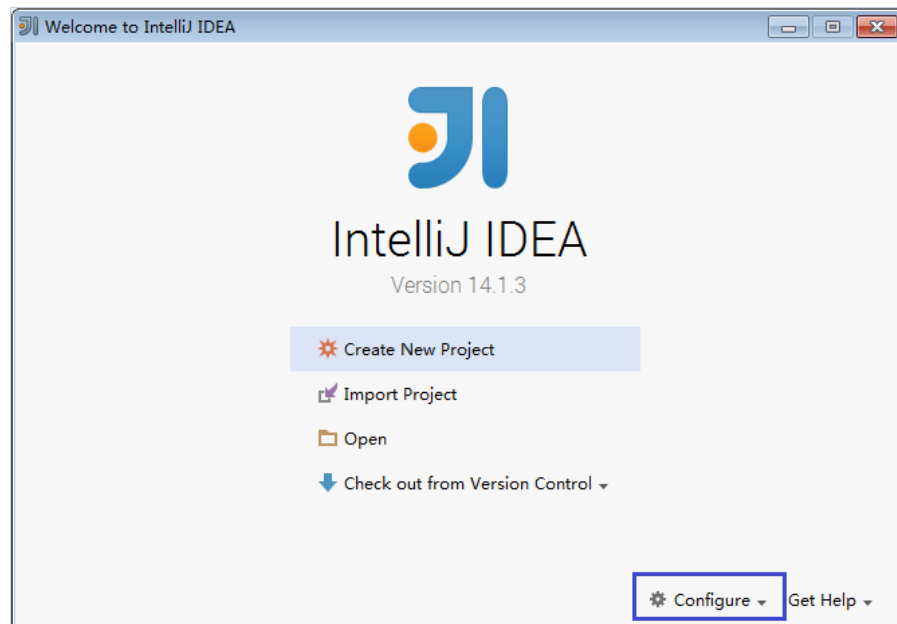
Figure 10-5 Choosing Configure
