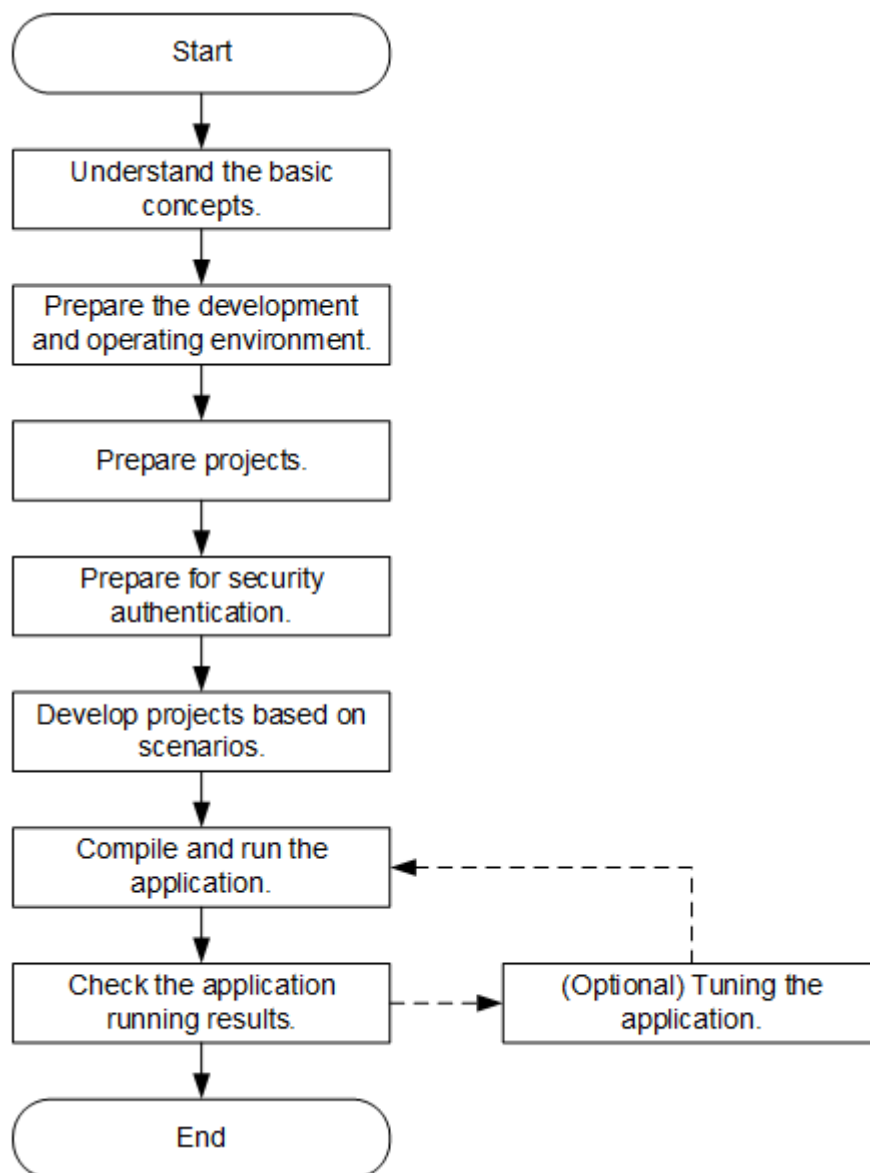
Figure 9-3 Development process
