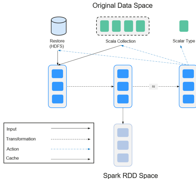
Figure 27-2 RDD operation
