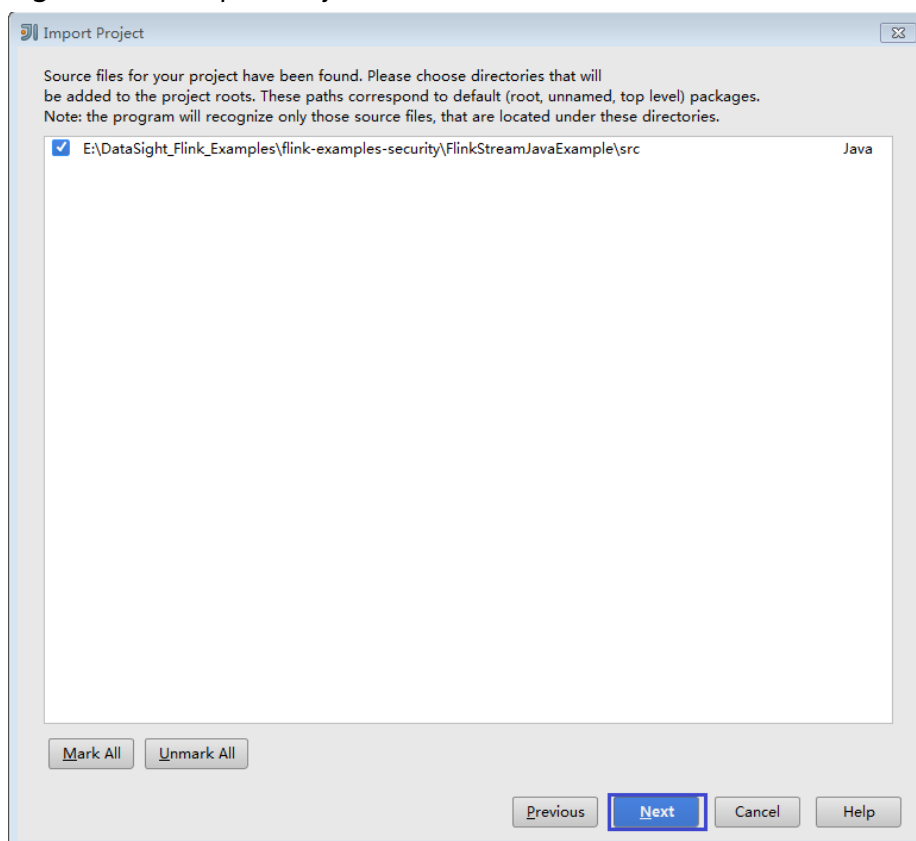
Figure 10-19 Import Project
