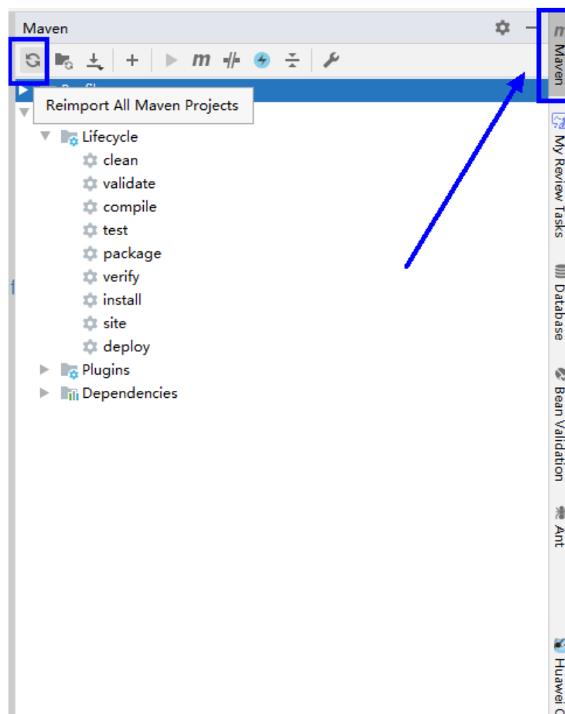
Figure 12-16 reimport projects
