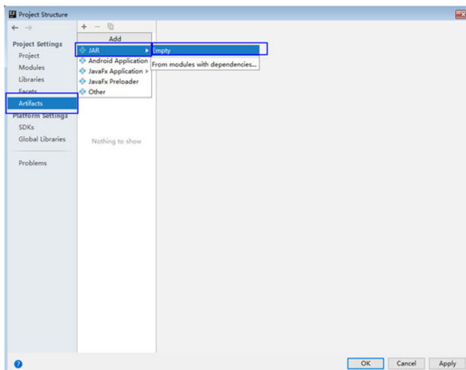
Figure 30-14 Adding Artifacts
