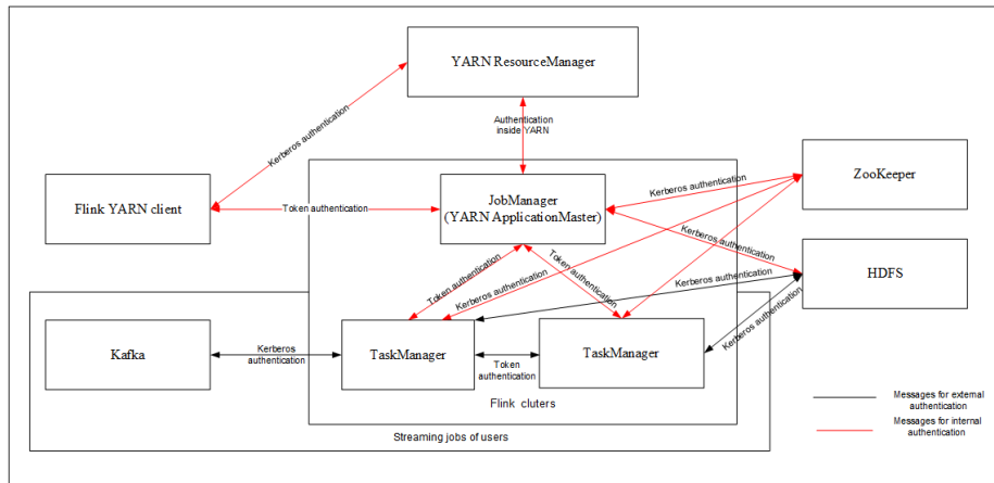
Figure 9-35 Authentication mode
