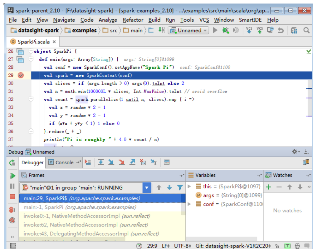
Figure 27-50 Debugging
