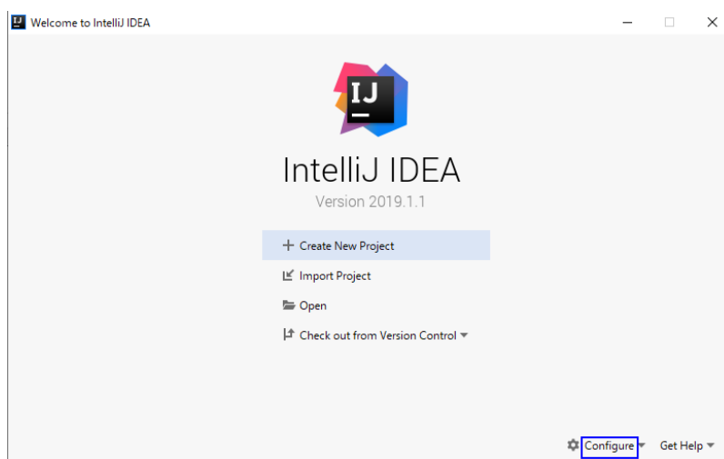
Figure 11-2 Quick Start
