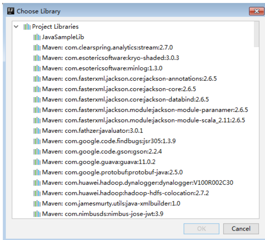
Figure 28-43 Choose Libraries
