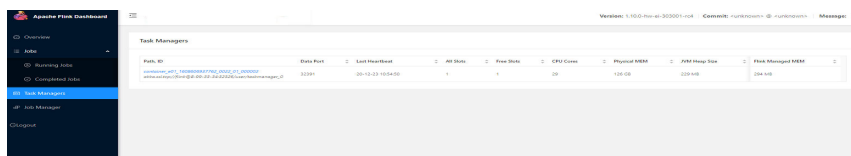
Figure 9-57 submitted task
