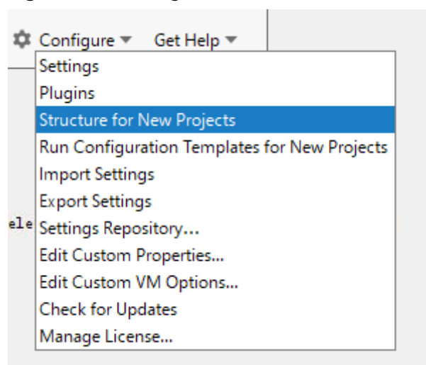
Figure 12-3 Configure
