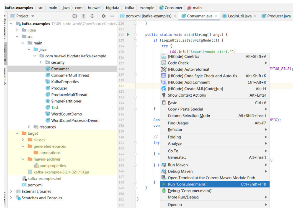
Figure 20-15 Running Consumer.java
