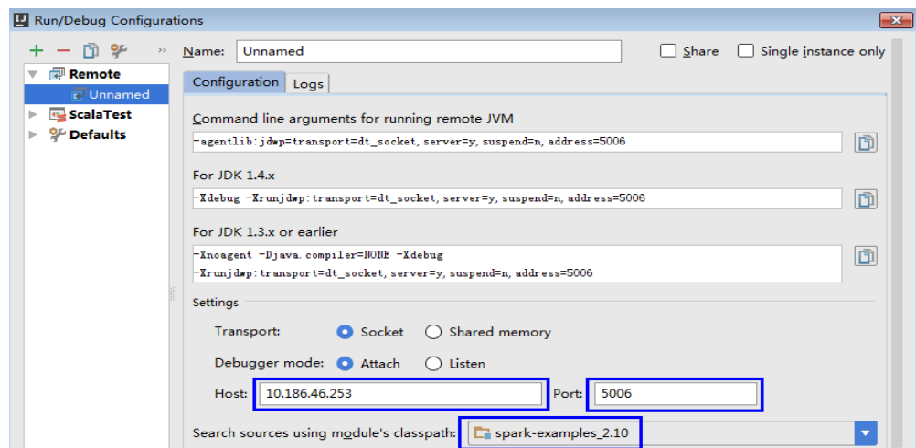
Figure 28-47 Configuring parameters
