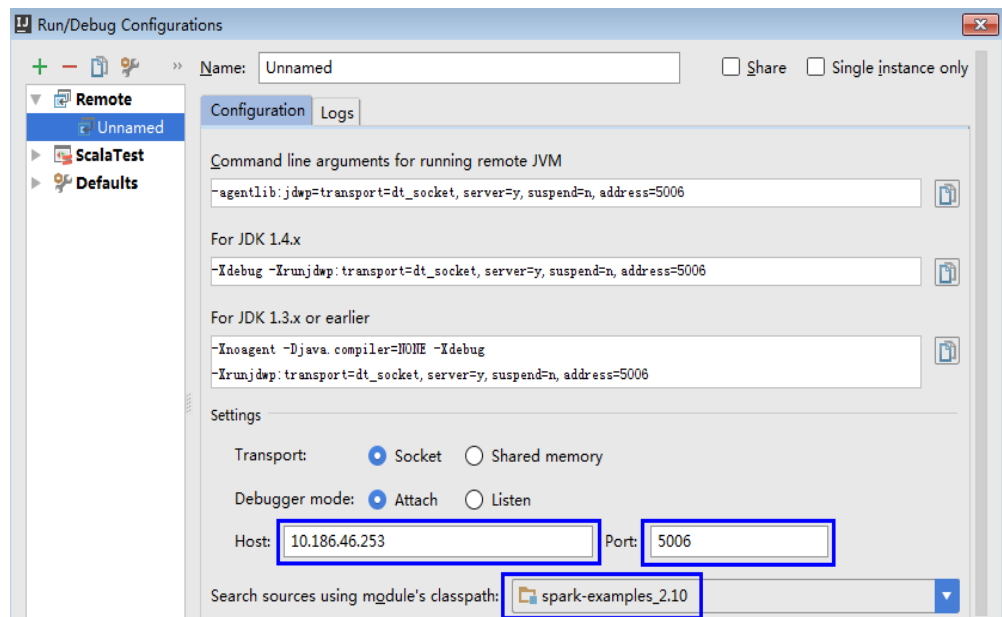
Figure 27-46 Choosing Remote
