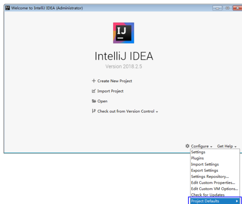
Figure 28-11 Configure
