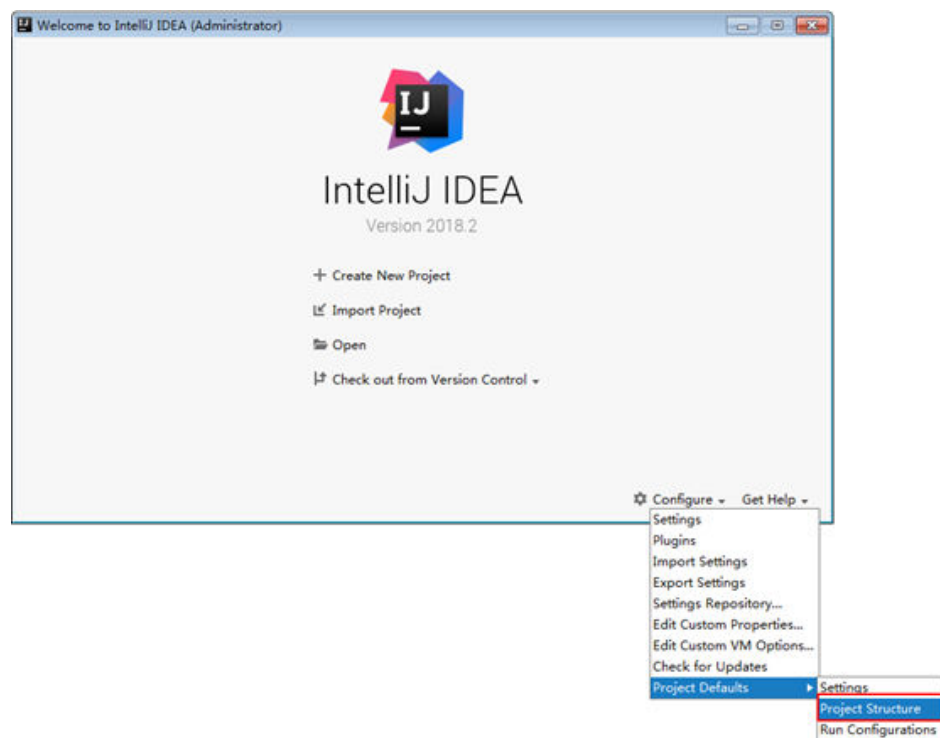
Figure 30-3 Configure
