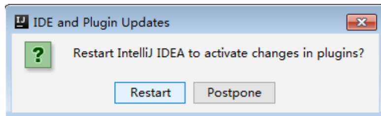
Figure 28-18 Plugins Changed
