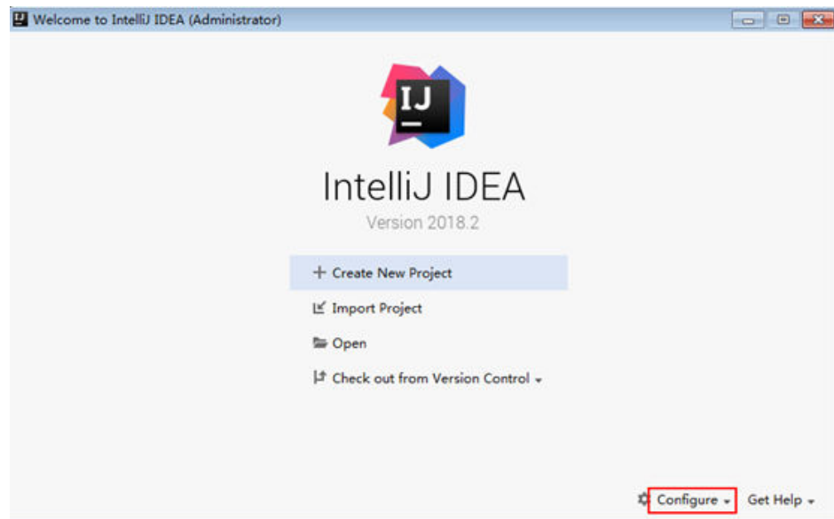
Figure 14-3 Quick Start
