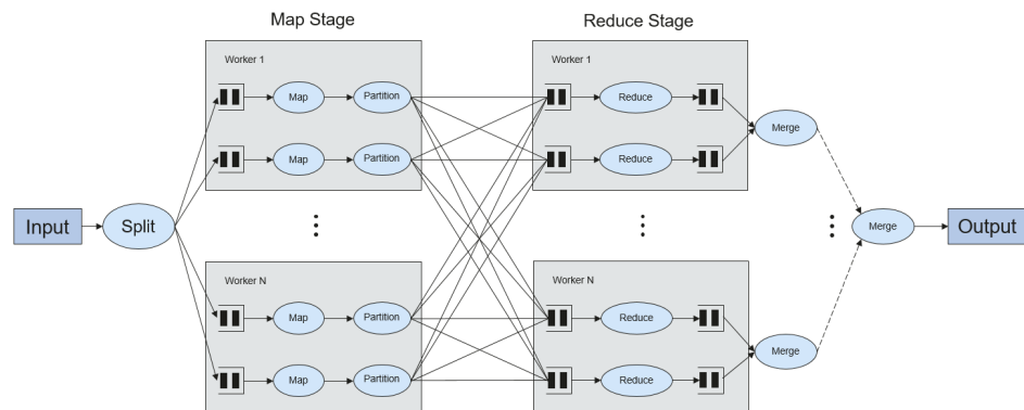
Figure 27-3 Algorithm process
