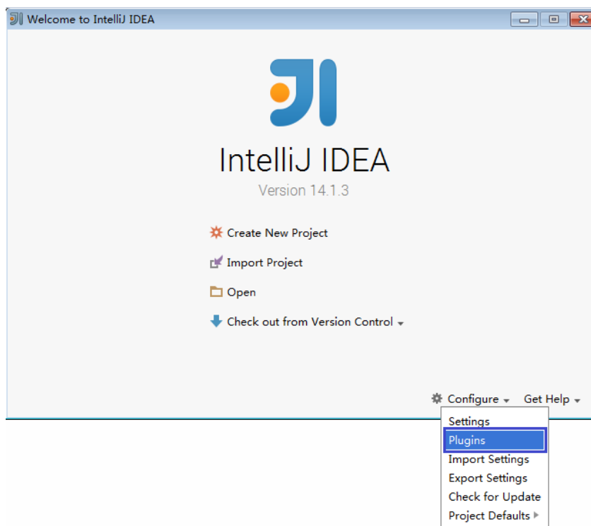
Figure 10-11 Plugins
