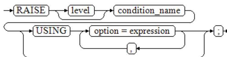
Figure 10-35 raise_condition::=
