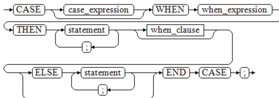
Figure 10-24 case_when::=
