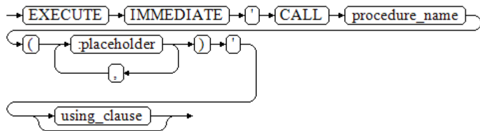
Figure 10-11 call_procedure::=
