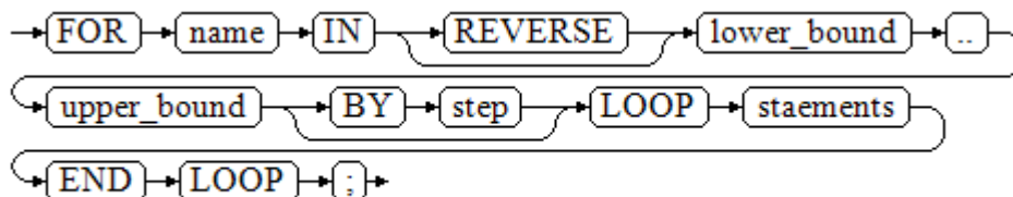
Figure 9-21 for_loop::=
