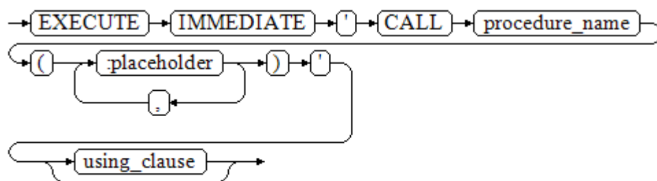
Figure 9-11 call_procedure::=
