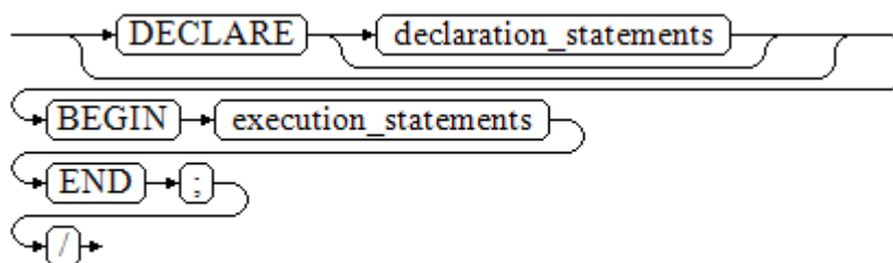
Figure 9-2 anonymous_block::=
