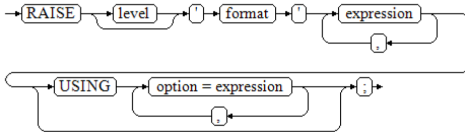
Figure 9-34 raise_format::=
