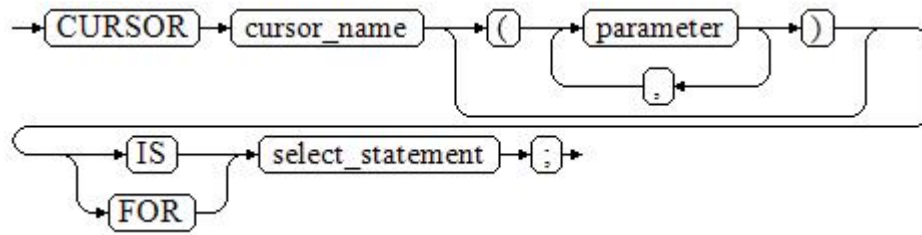
Figure 9-26 static_cursor_define::=
