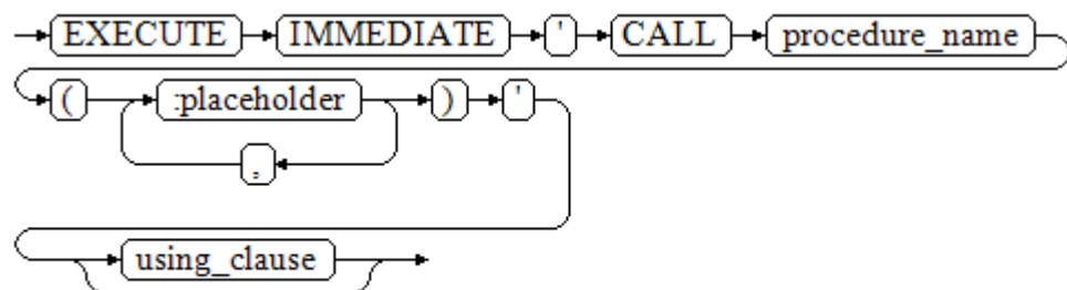
Figure 10-12 call_procedure::=
