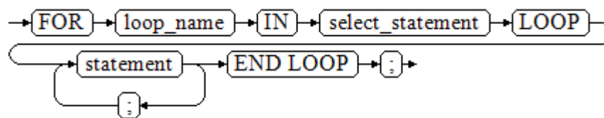
Figure 10-34 FOR_AS_loop::=
