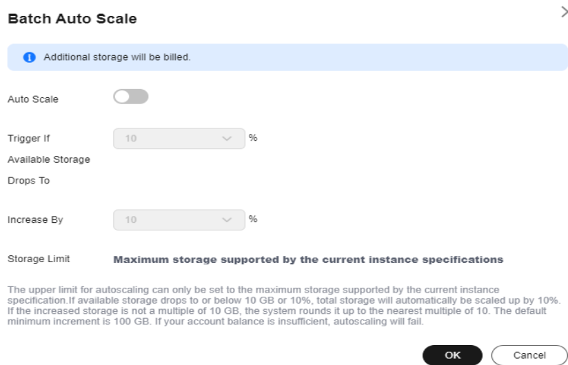
Figure 3-26 Batch Auto Scale
