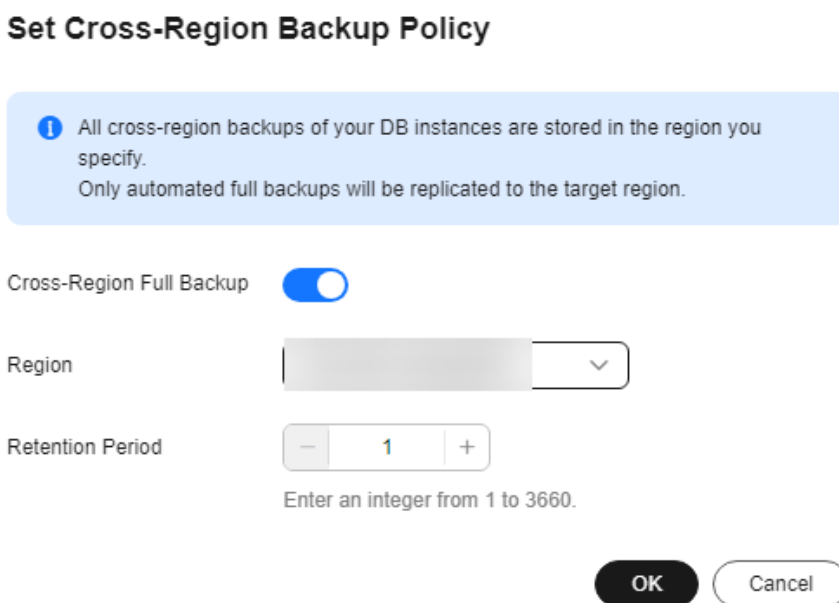
Figure 3-60 Setting a cross-region backup policy
