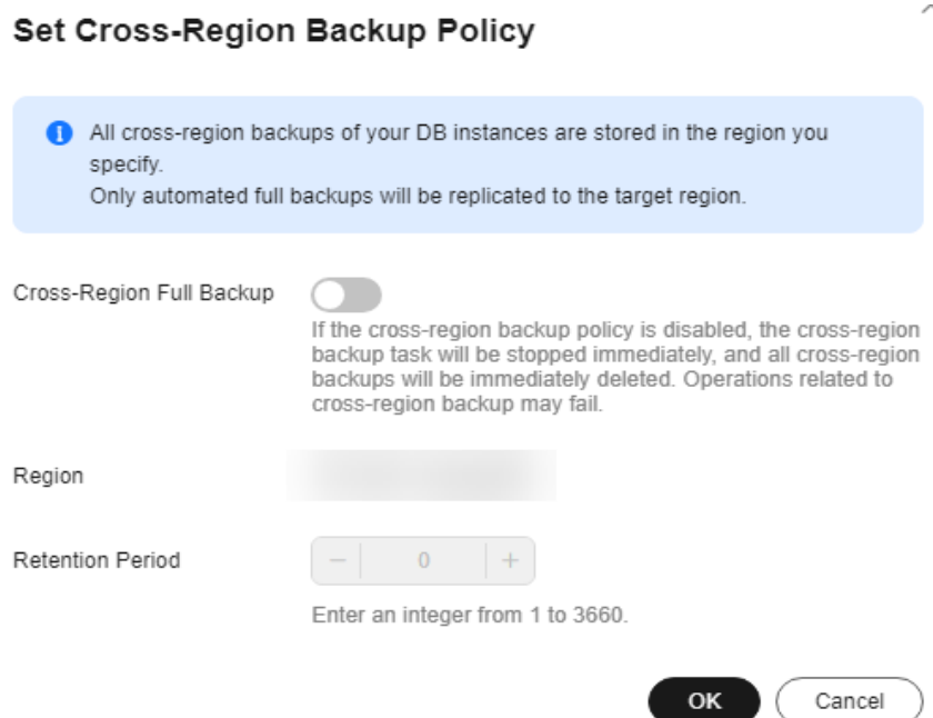
Figure 3-63 Disabling cross-region backup
