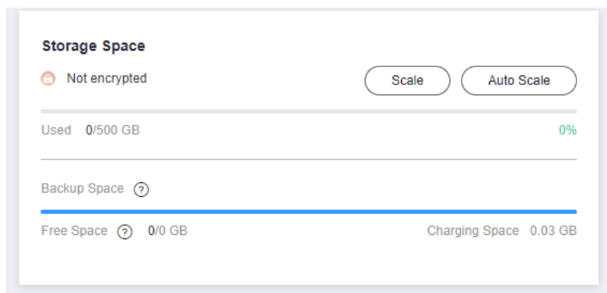
Figure 3-23 Auto Scale
