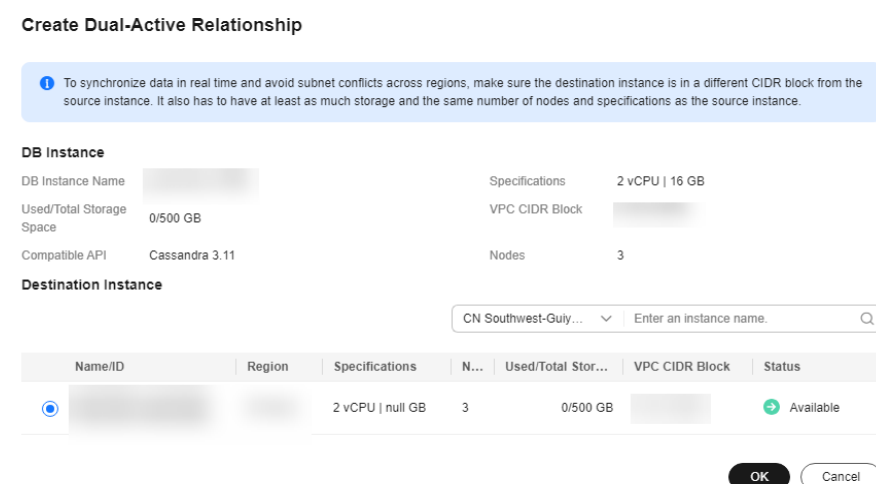
Figure 3-55 Selecting the destination instance
