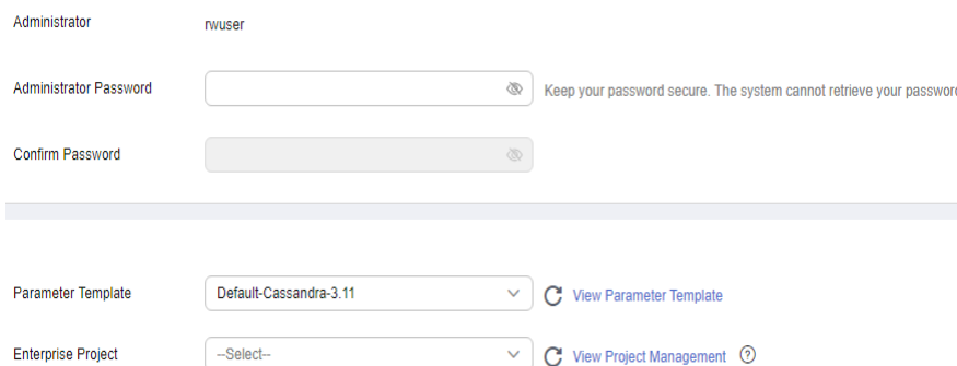
Figure 3-6 Database configuration
