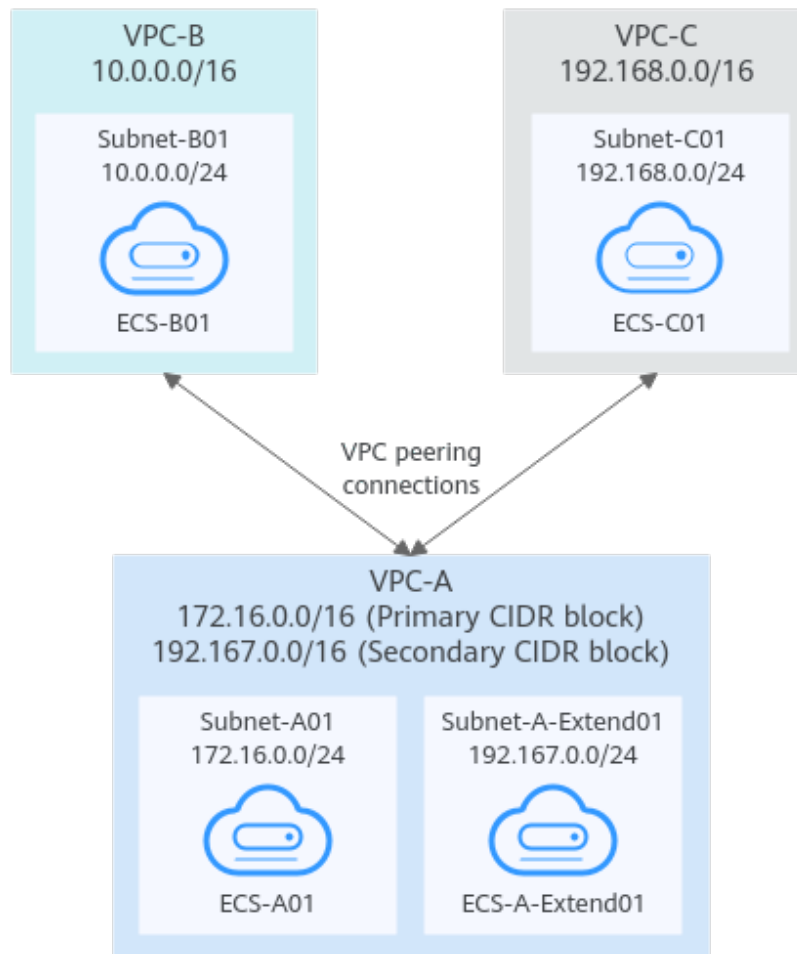
Figure 13-8 Networking diagram (IPv4)
