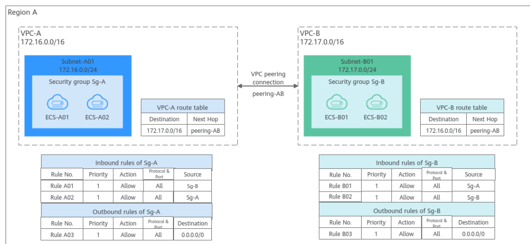
Figure 6-4 Security group examples (allowing communications between ECSs in two VPCs connected by a VPC peering connection )
