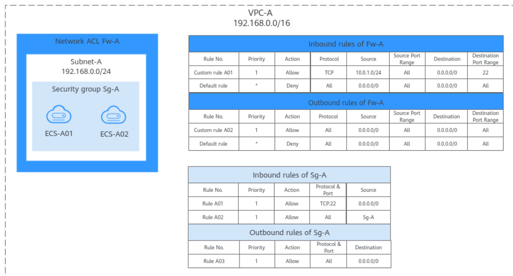
Figure 6-5 Network ACL examples (allowing traffic from specific IP addresses to the instances in a subnet)
