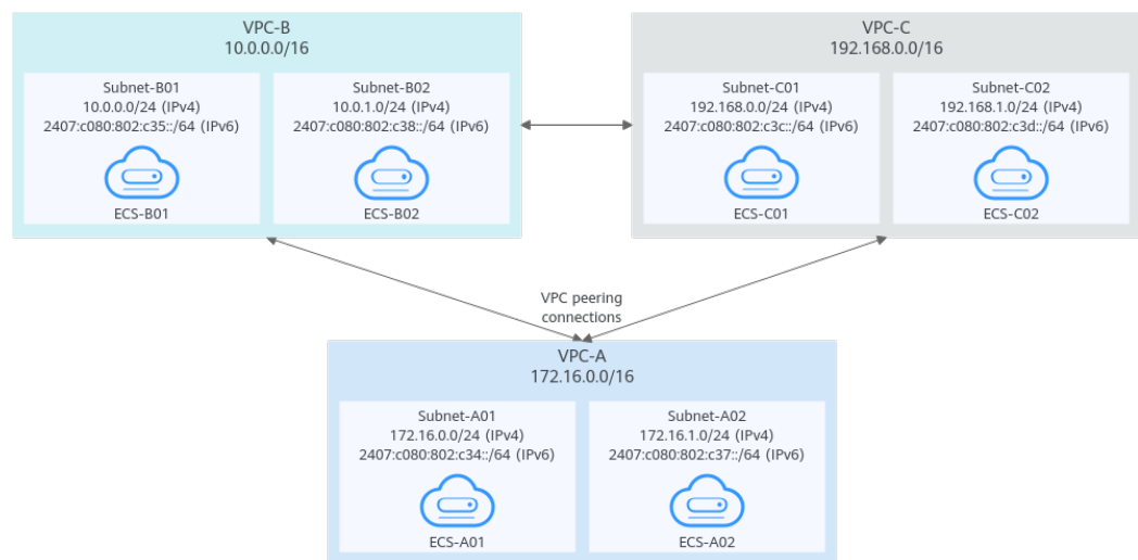
Figure 13-5 Networking diagram (IPv6)
