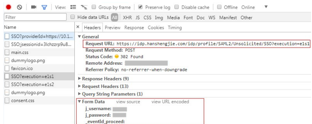
Figure 5-5 Authentication information (1)
