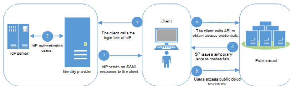
Figure 5-3 Flowchart (IdP-initiated)
