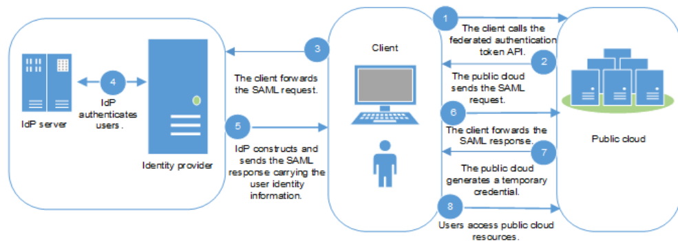
Figure 5-2 Flowchart (SP-initiated)
