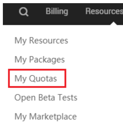
Figure 1-2 My Quotas
