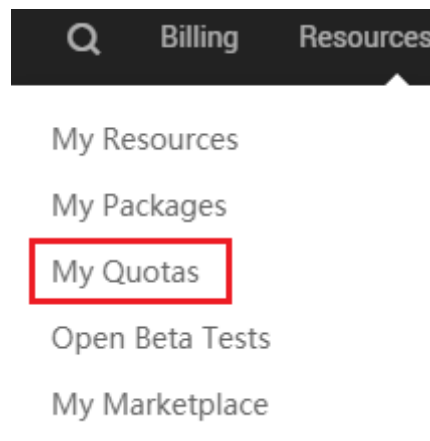
Figure 1-3 My Quotas
