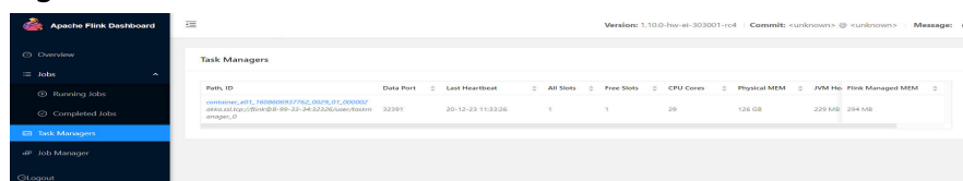
Figure 7-52 submitted task
