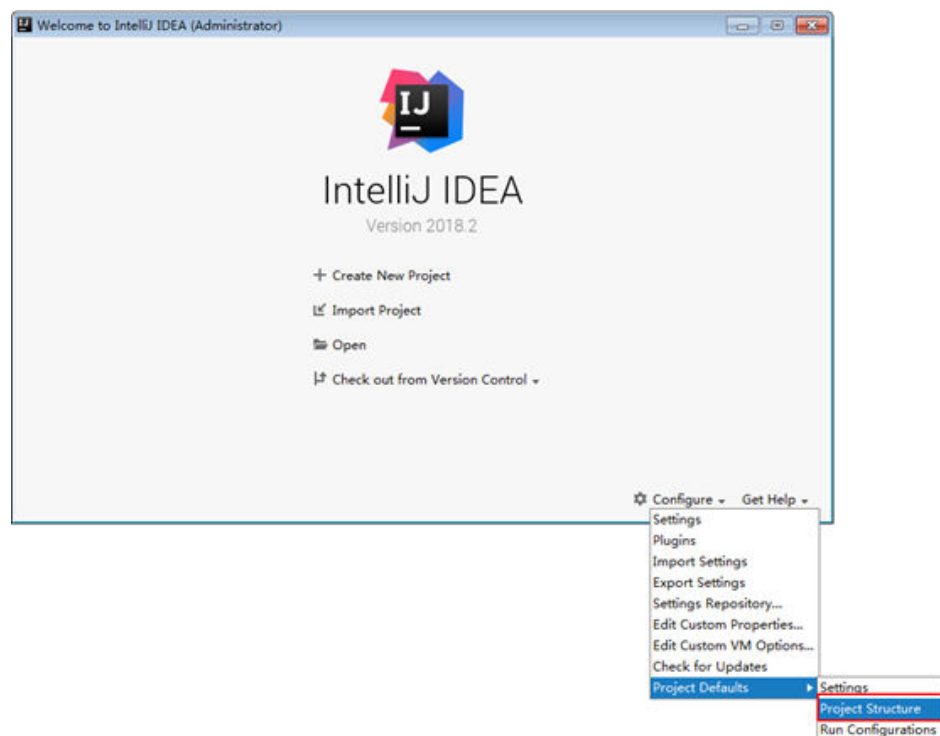
Figure 18-3 Configure
