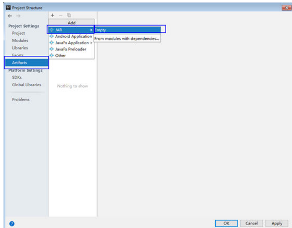
Figure 29-12 Adding Artifacts
