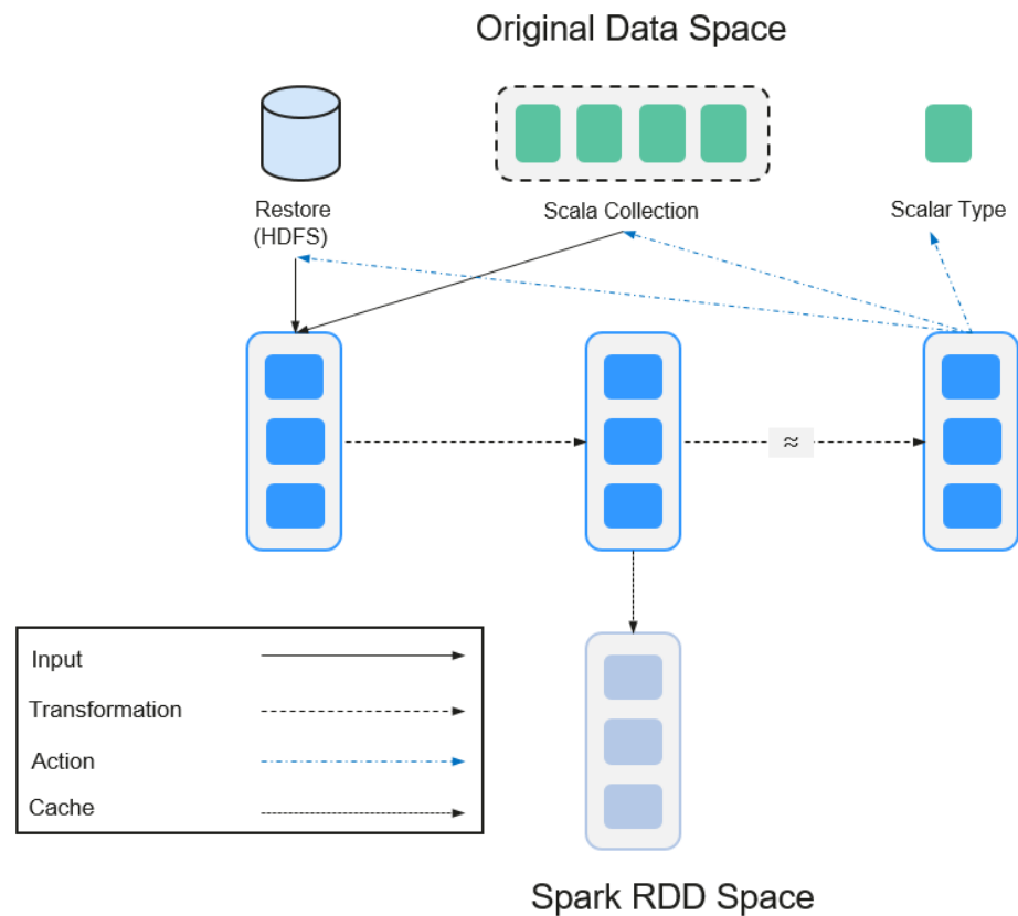
Figure 27-2 RDD operation
