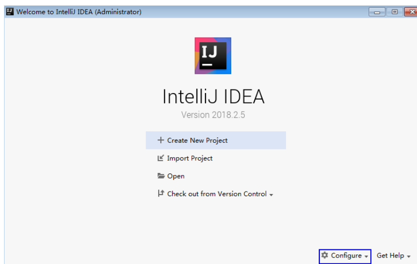
Figure 27-10 Quick Start
