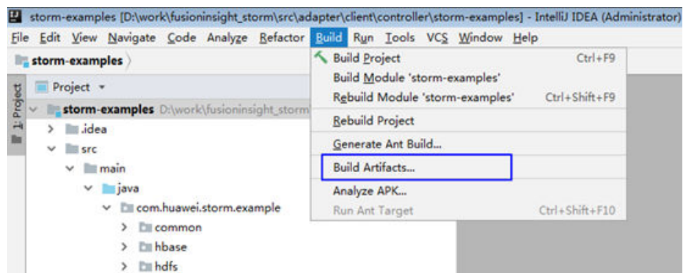
Figure 30-15 Build Artifacts
