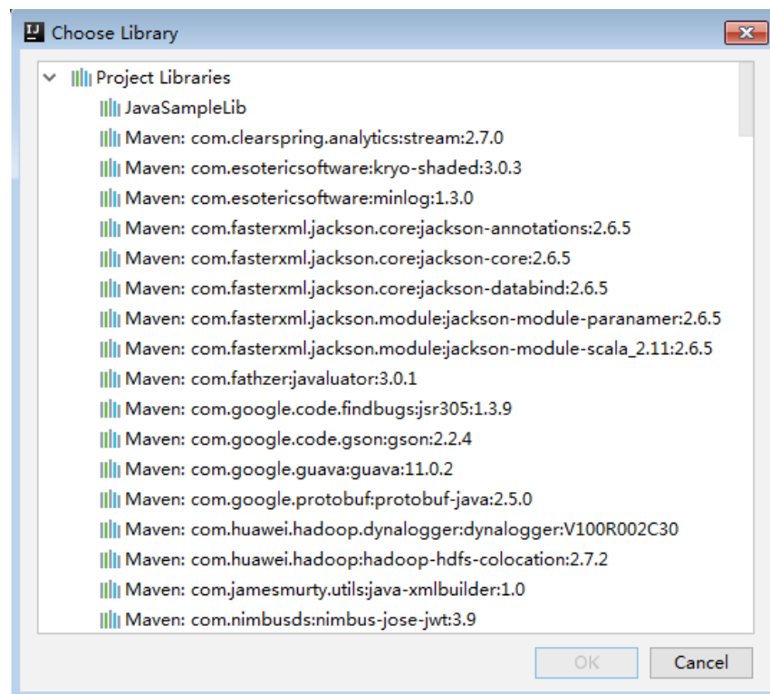
Figure 27-43 Choose Libraries
