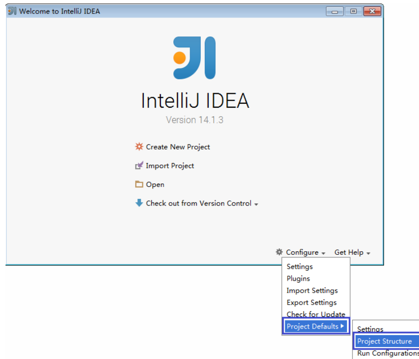
Figure 8-7 Project Defaults
