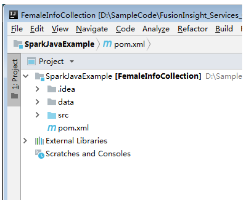
Figure 27-24 Imported project
