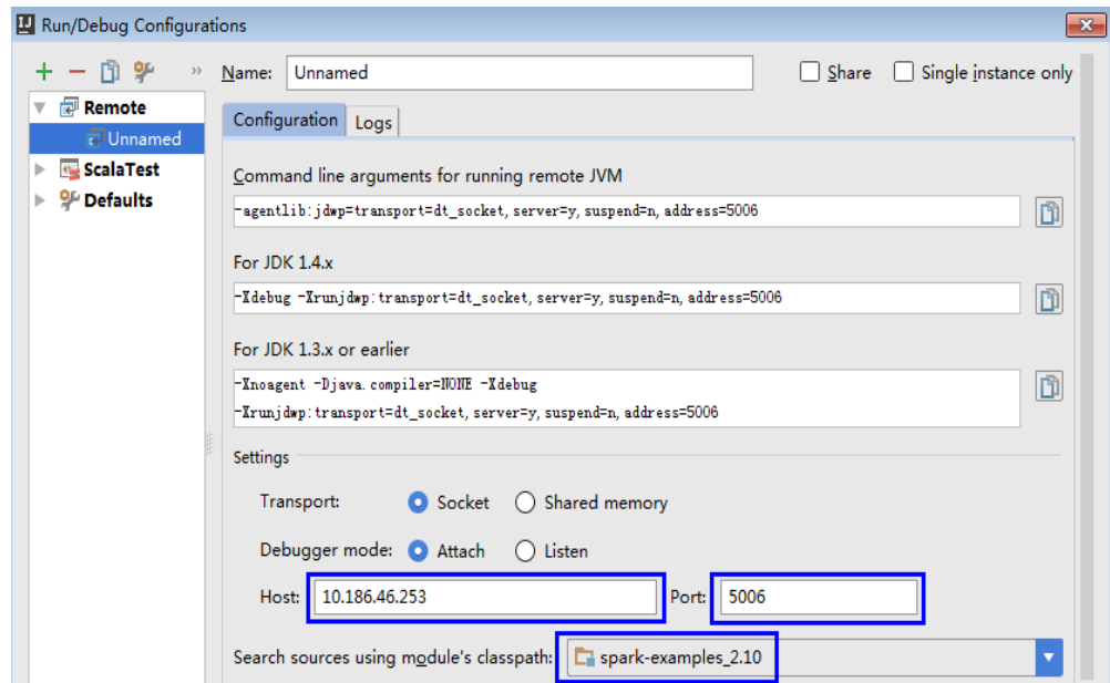
Figure 28-45 Choosing Remote
