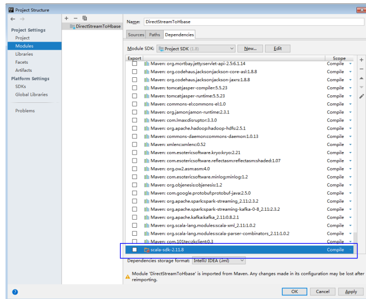
Figure 28-30 Successful configuration
