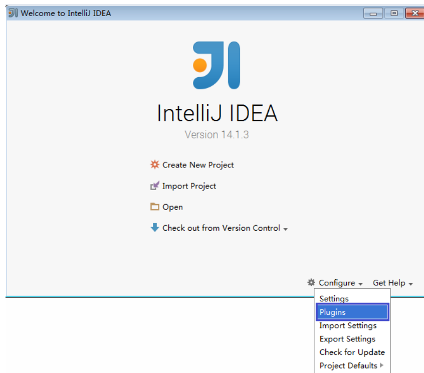
Figure 7-11 Plugins
