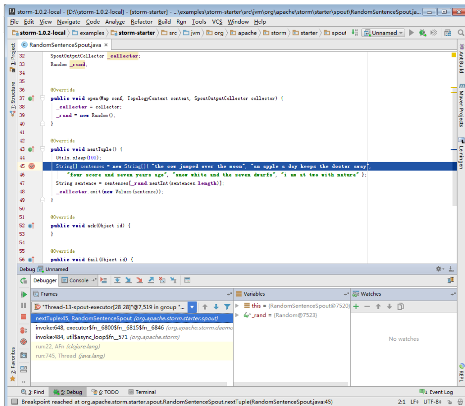
Figure 29-23 Debugging
