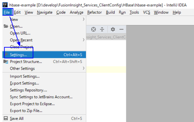
Figure 9-13 Settings
