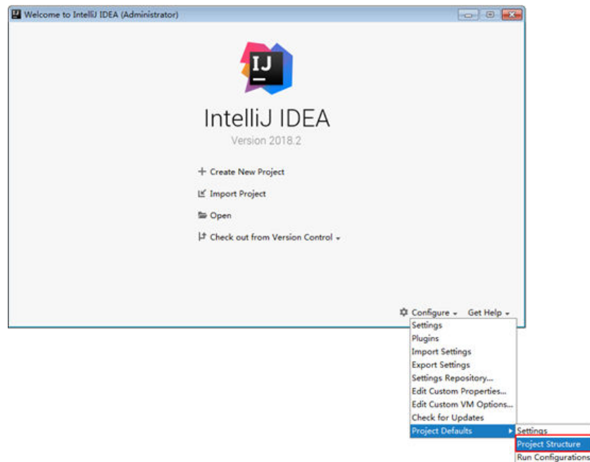
Figure 5-3 Configure
