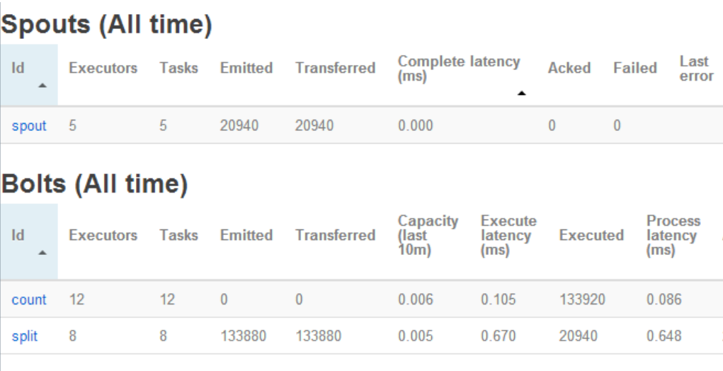
Figure 30-18 Total volume of data sent by the Storm application operators
