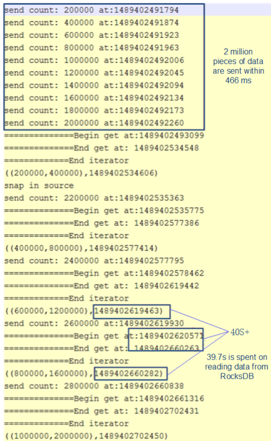
Figure 7-68 Time monitoring
