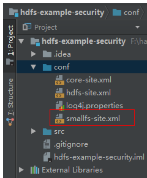
Figure 11-4 Importing smallfs-site.xml
