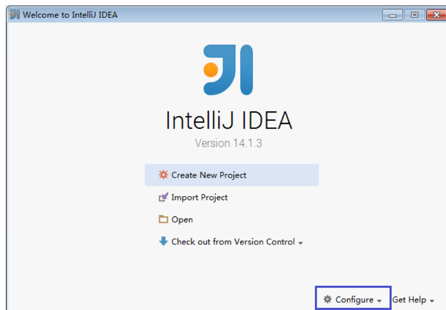
Figure 7-5 Choosing Configure
