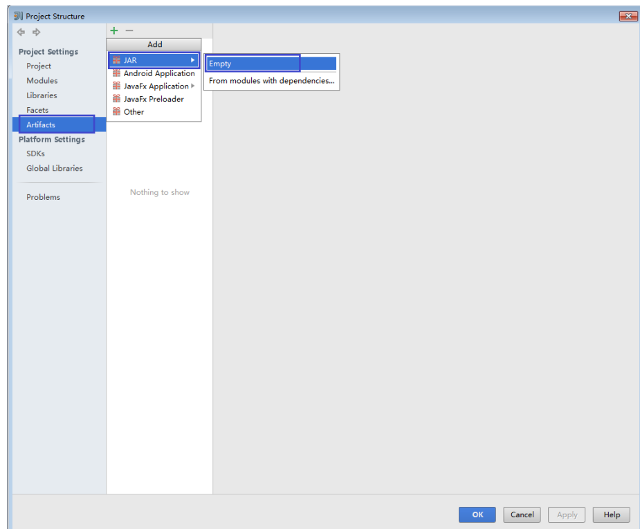
Figure 7-40 Adding Artifacts
