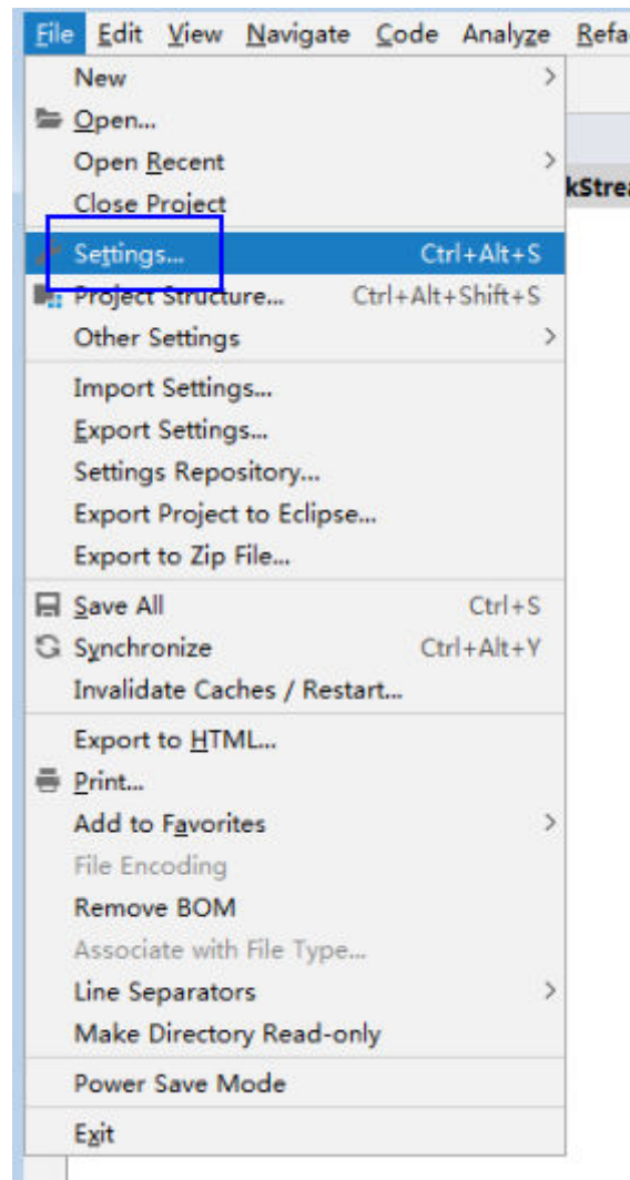
Figure 27-31 Choose Settings
