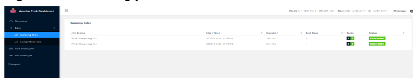
Figure 7-57 running jobs
