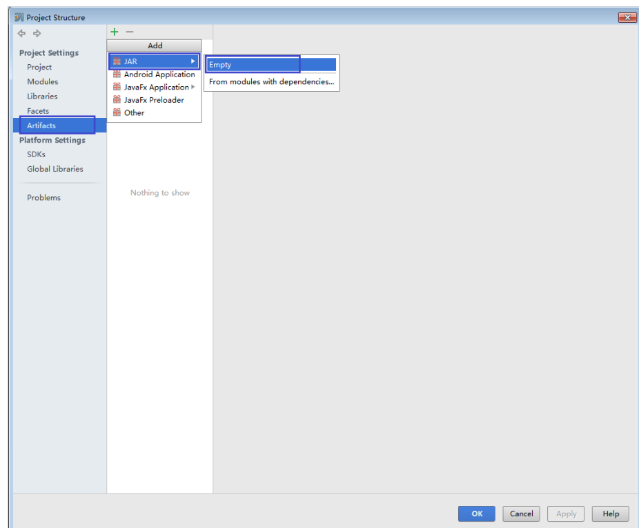
Figure 8-38 Adding Artifacts
