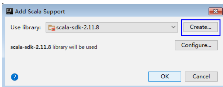
Figure 27-27 Create...
