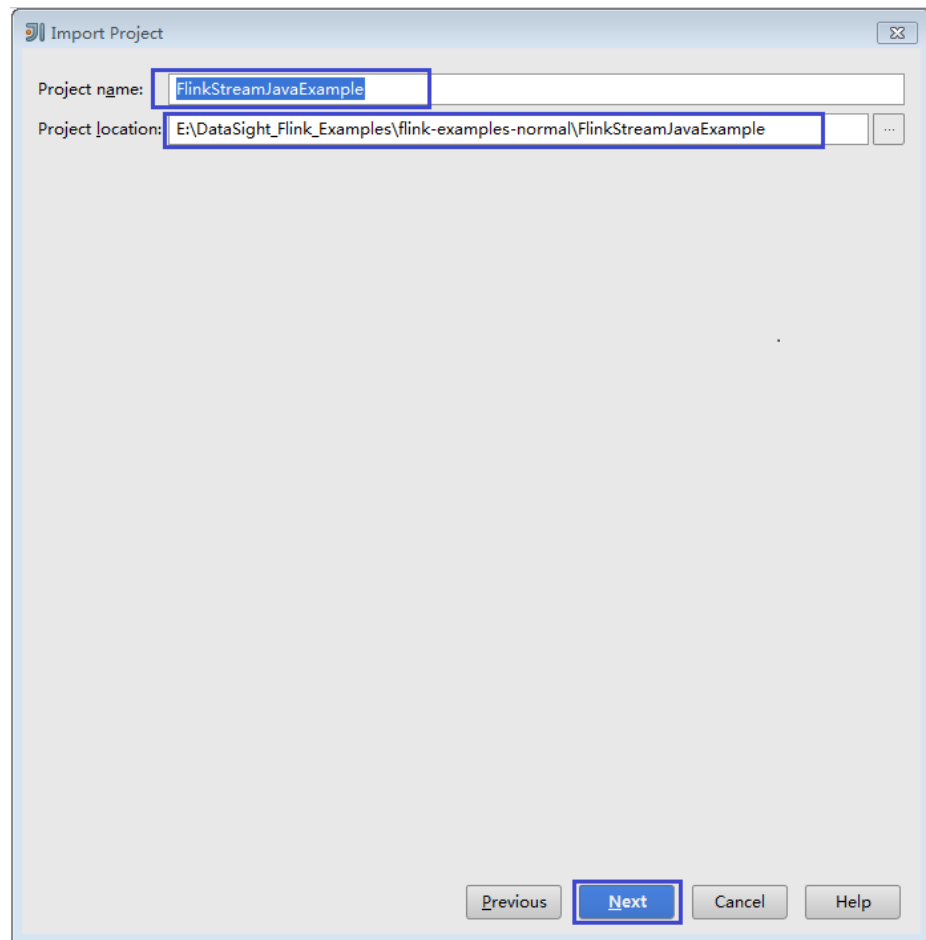
Figure 8-18 Import Project
