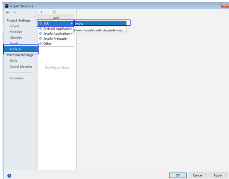
Figure 17-11 Add Artifacts
