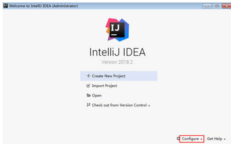
Figure 30-2 Quick Start
