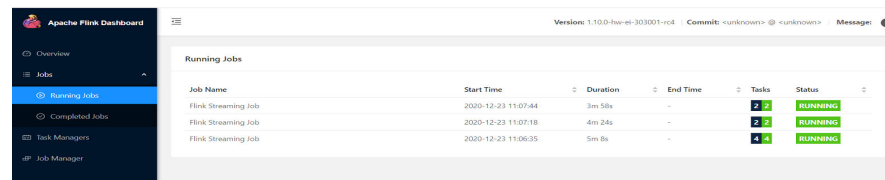
Figure 7-48 submitted Tasks
