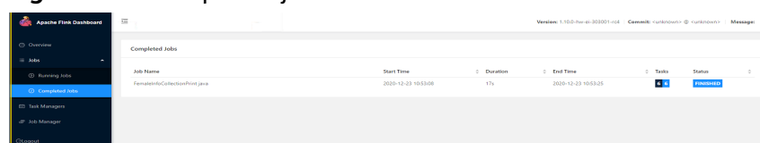
Figure 7-54 completed job
