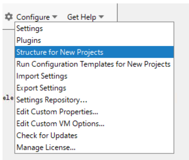
Figure 9-3 Configure
