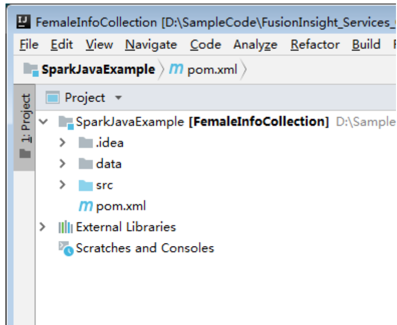
Figure 28-24 Imported project
