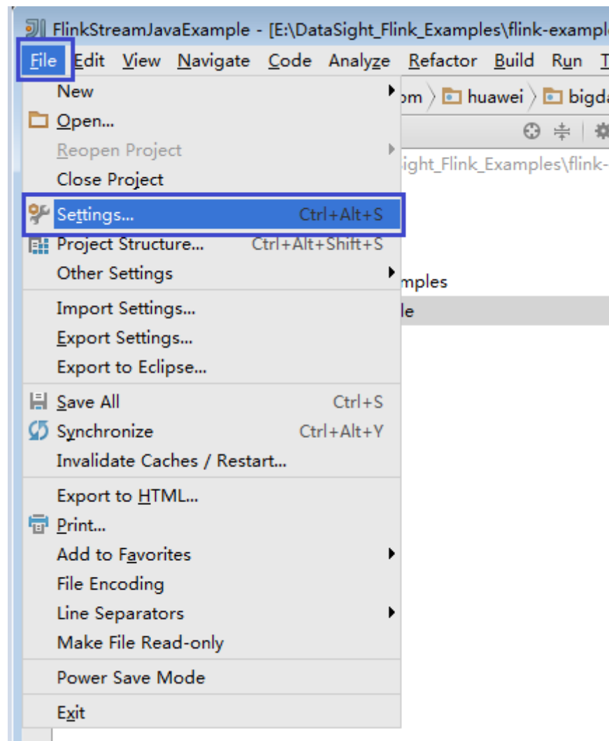
Figure 7-28 Choosing Settings
