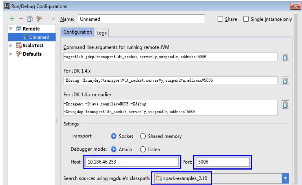
Figure 27-45 Choosing Remote
