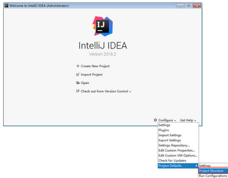
Figure 6-3 Configure
