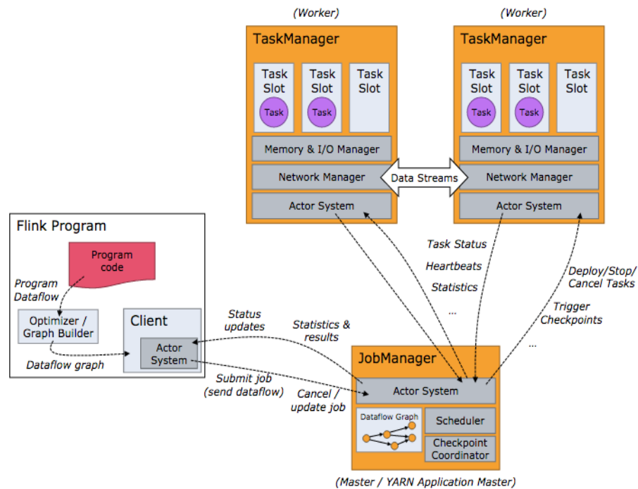
Figure 7-2 Flink architecture
