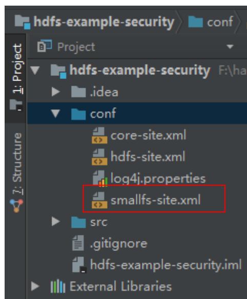
Figure 12-4 Importing smallfs-site.xml
