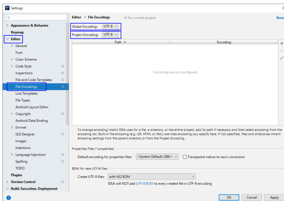
Figure 10-16 File Encodings
