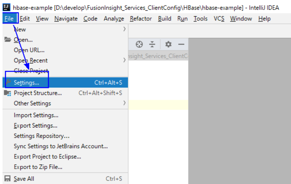
Figure 10-15 Settings
