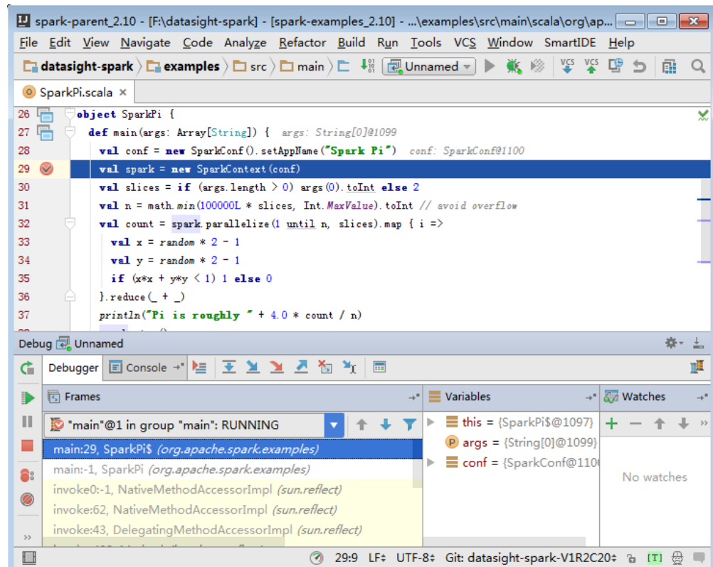
Figure 27-49 Debugging
