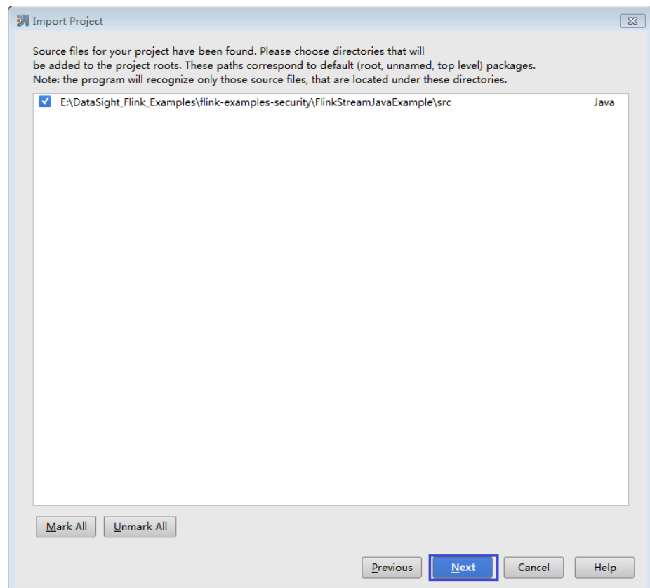
Figure 7-19 Import Project
