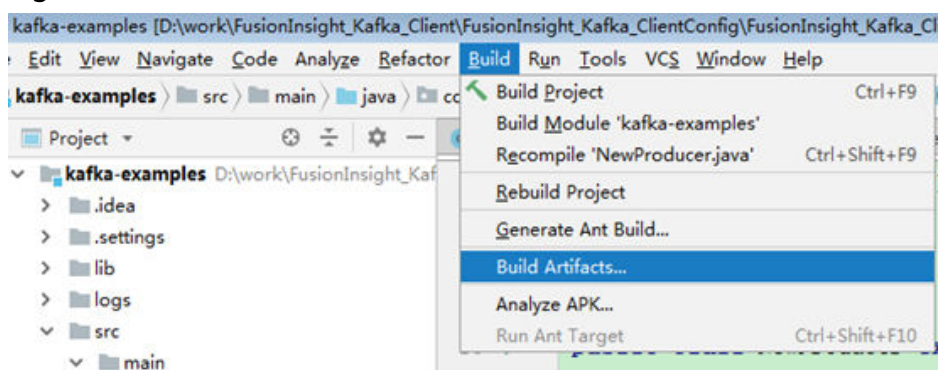
Figure 18-14 Build Artifacts
