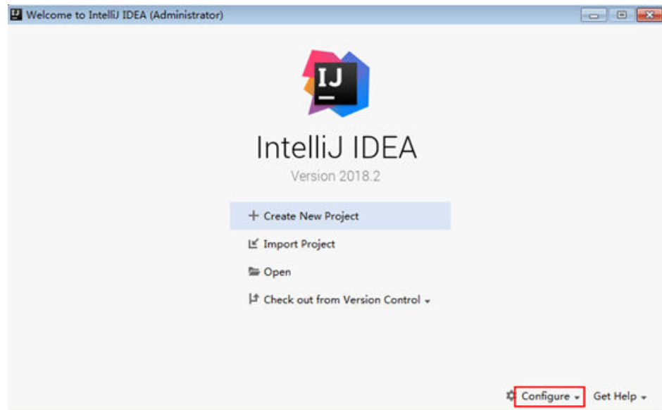
Figure 18-2 Quick Start
