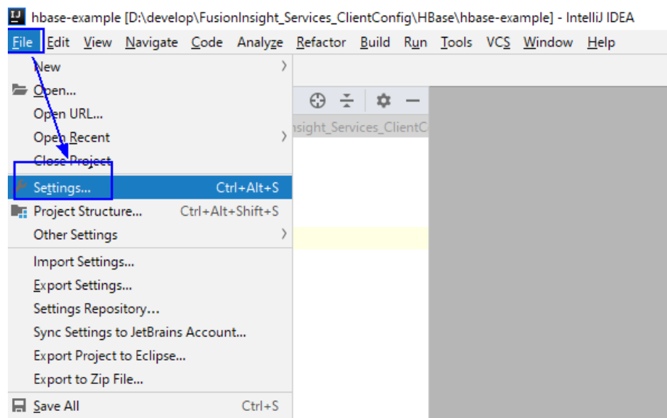
Figure 9-15 Settings
