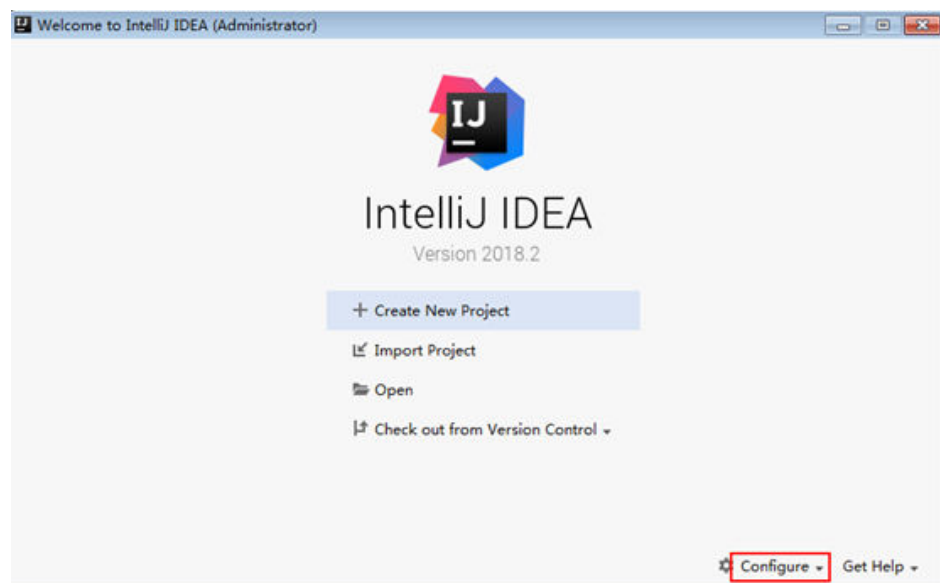
Figure 17-2 Quick Start
