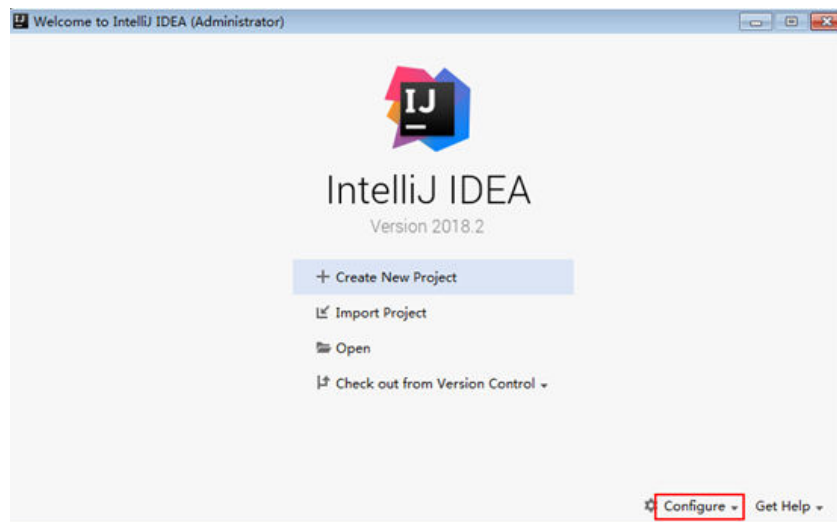
Figure 6-2 Quick Start
