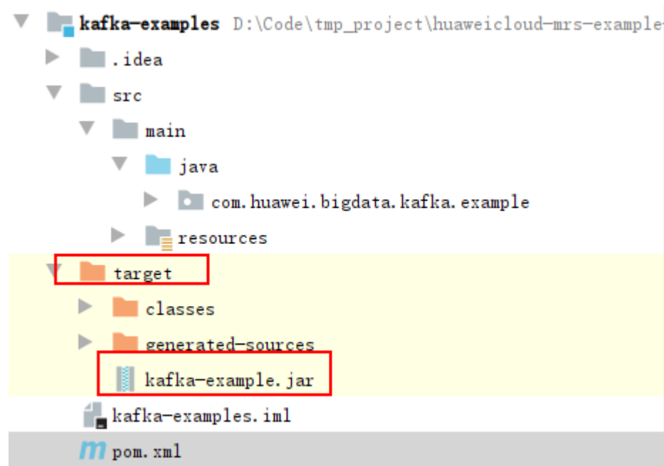
Figure 17-16 File location
