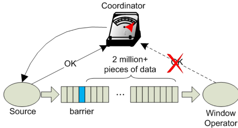
Figure 7-69 Relationship
