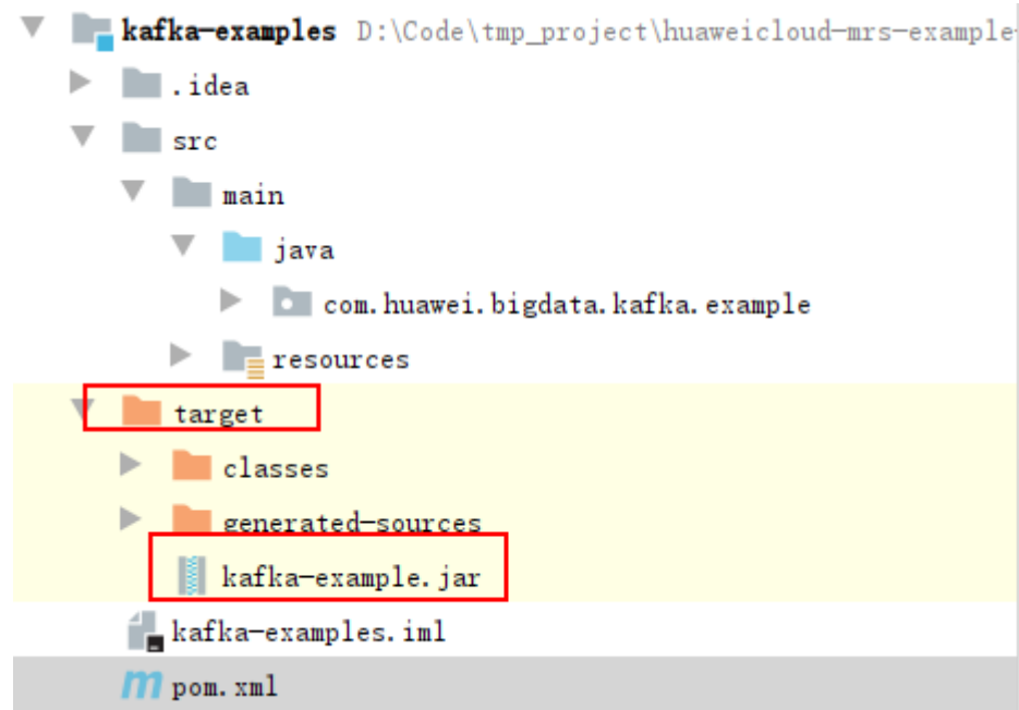
Figure 18-16 File Location
