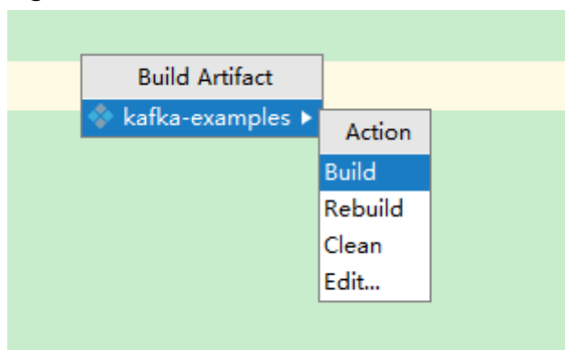
Figure 18-15 Build
