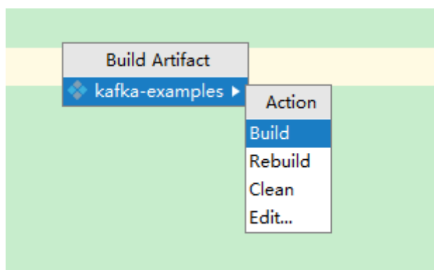
Figure 17-15 Build
