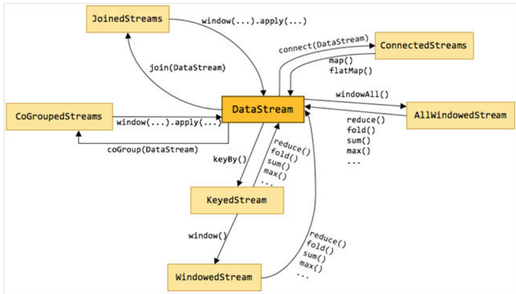
Figure 8-59 Conversion of Flink stream types
