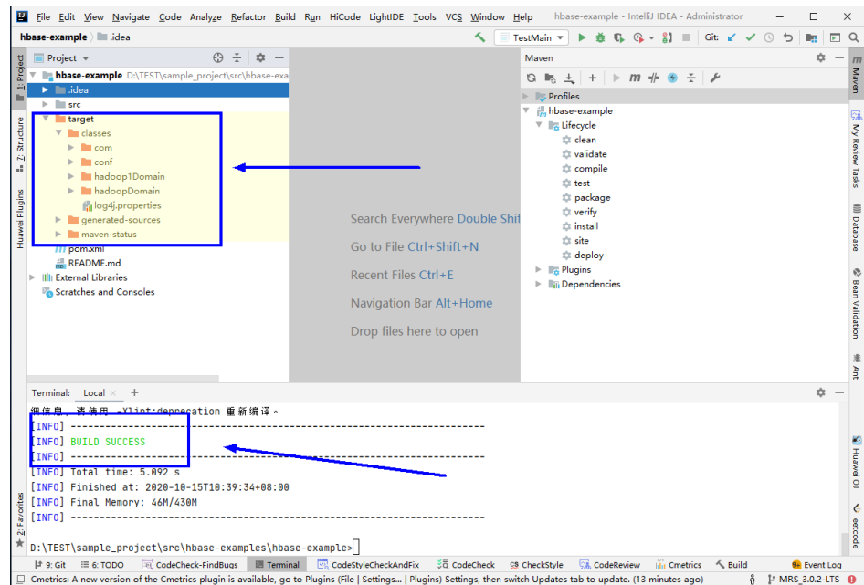
Figure 9-21 Compilation completed
