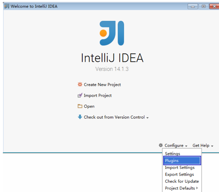
Figure 8-11 Plugins
