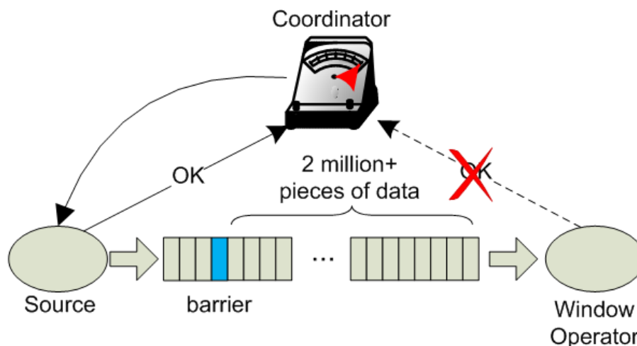
Figure 8-64 Relationship
