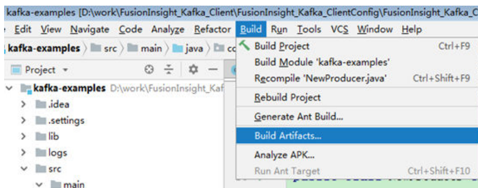
Figure 17-14 Build Artifacts
