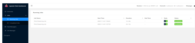
Figure 8-52 Running jobs
