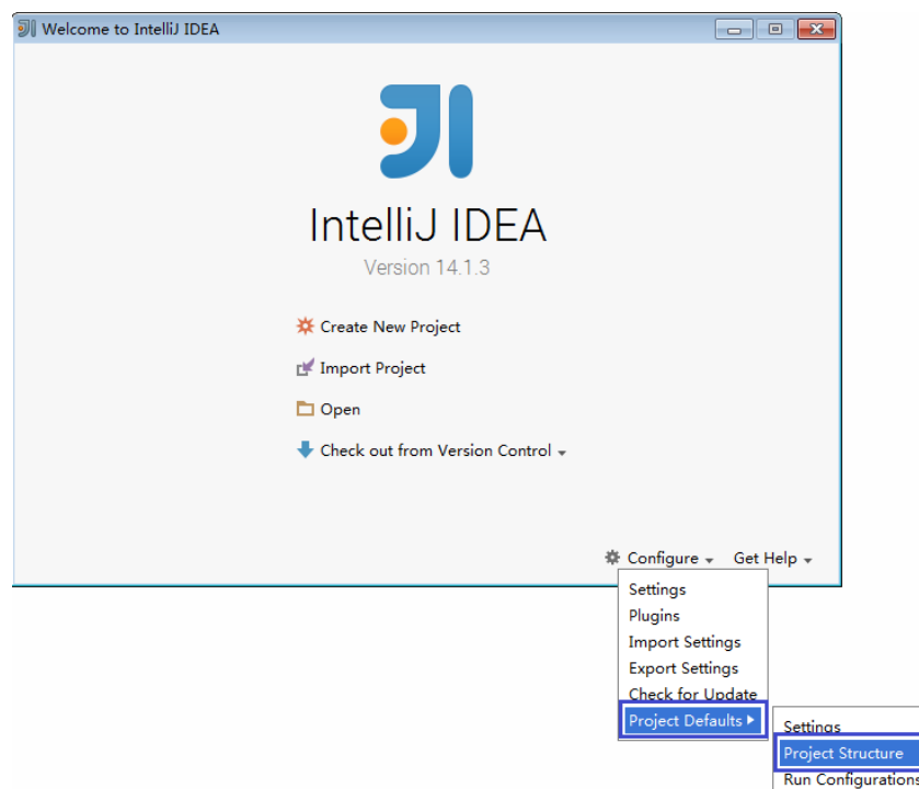
Figure 7-7 Project Defaults
