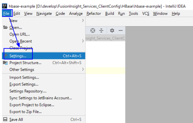
Figure 10-13 Settings
