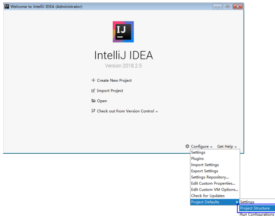
Figure 27-12 Project Defaults
