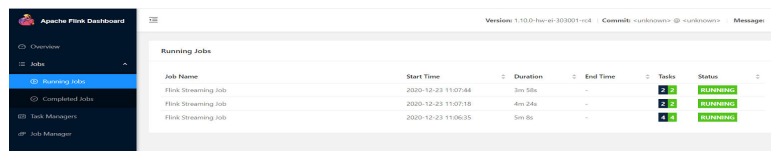
Figure 8-45 Running jobs
