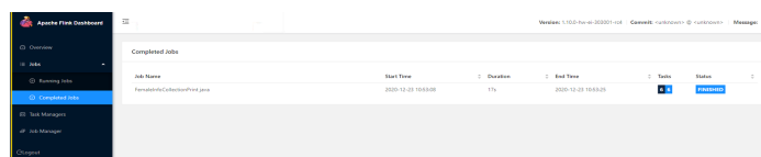
Figure 8-49 Completed job
