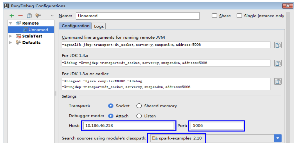
Figure 28-46 Configuring parameters
