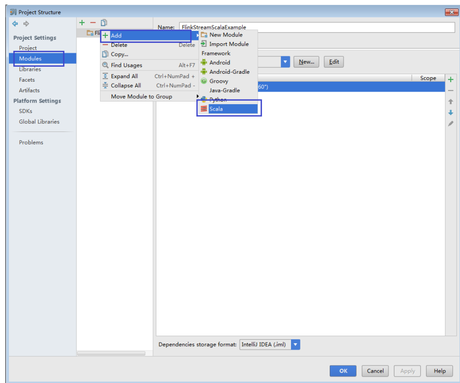
Figure 7-22 Selecting Scala
