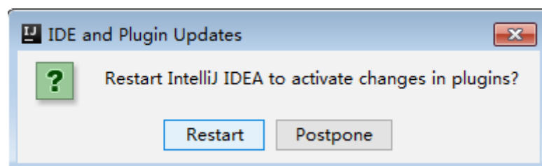
Figure 27-18 Plugins Changed
