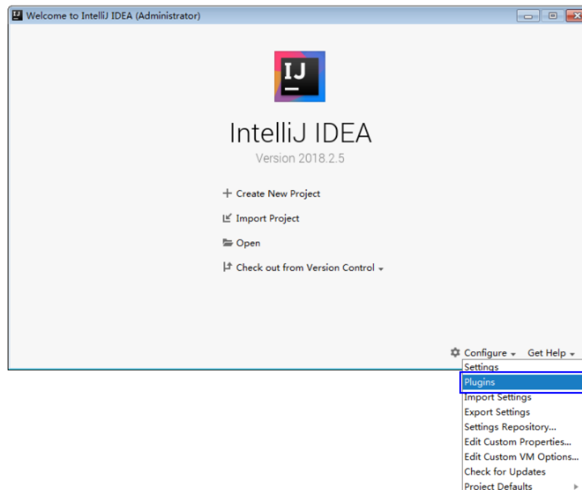
Figure 27-16 Plugins
