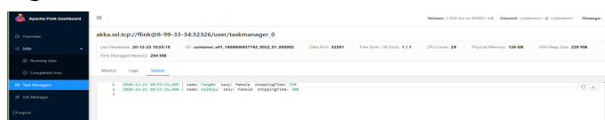
Figure 8-51 Execution result
