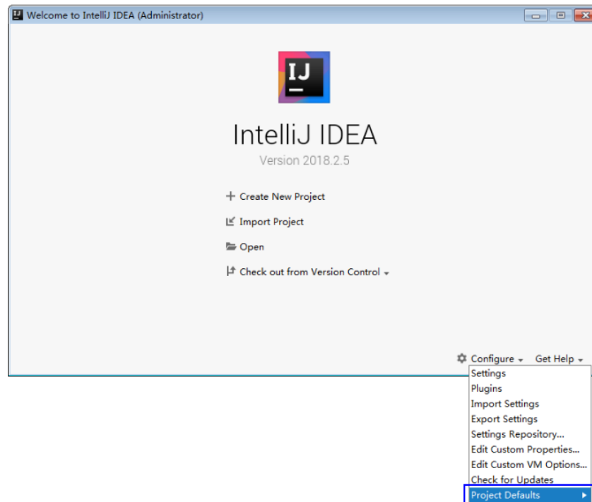
Figure 27-11 Configure
