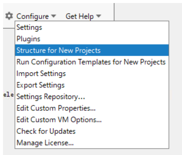
Figure 10-3 Configure
