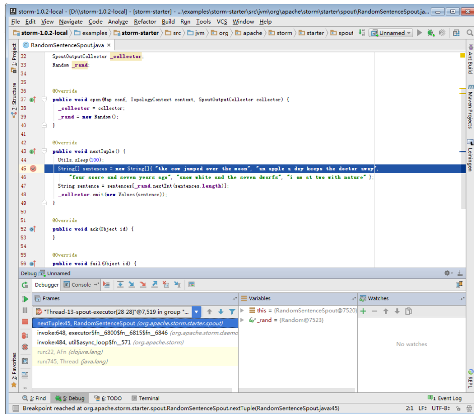
Figure 30-23 Debugging
