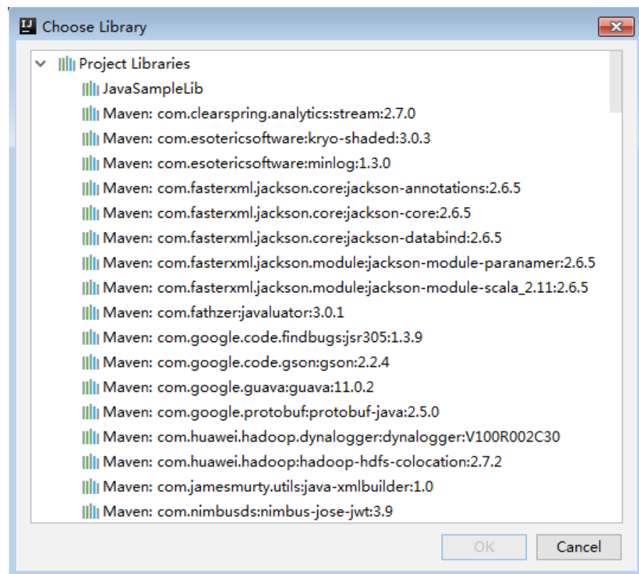
Figure 28-43 Choose Libraries
