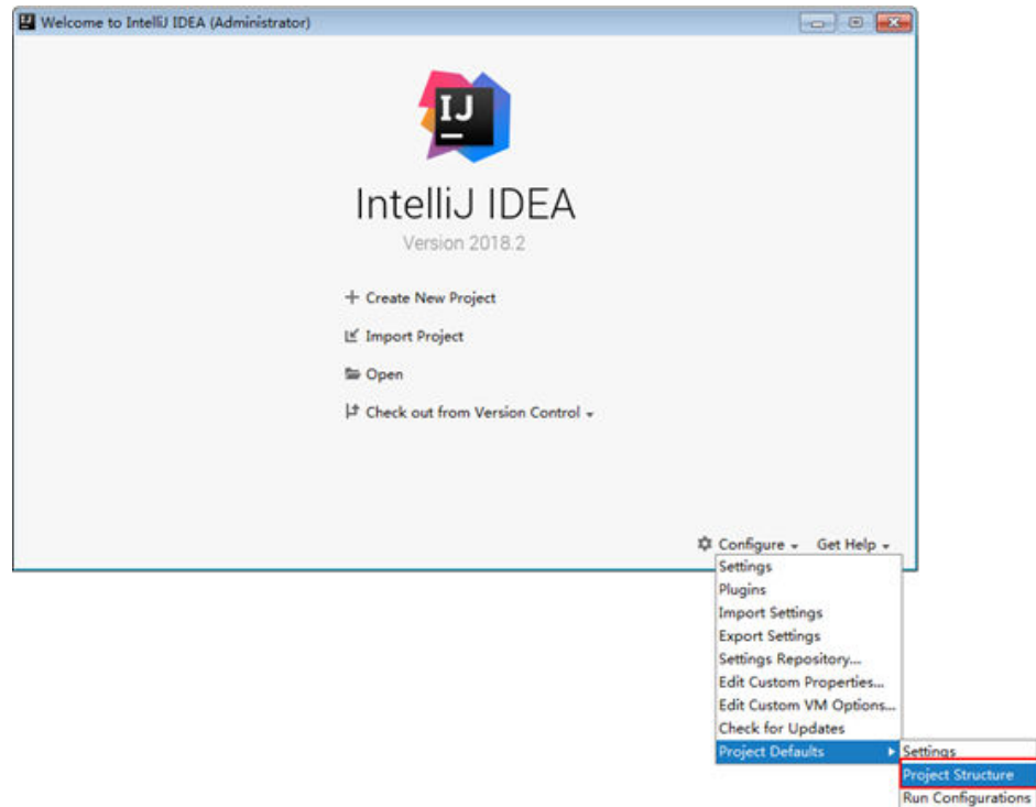
Figure 17-3 Configure
