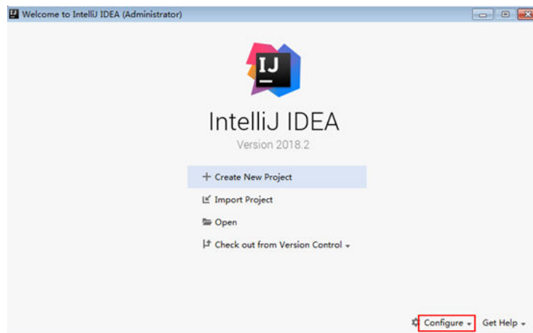
Figure 5-2 Quick Start
