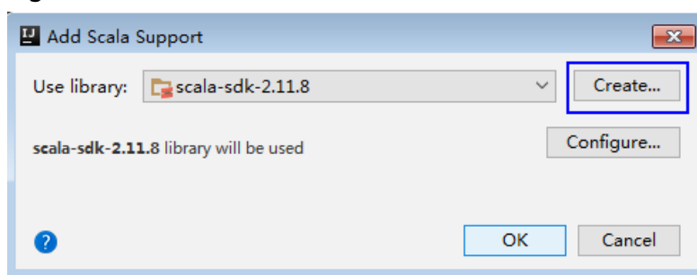
Figure 28-27 Create...
