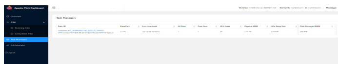
Figure 8-50 Submitted task
