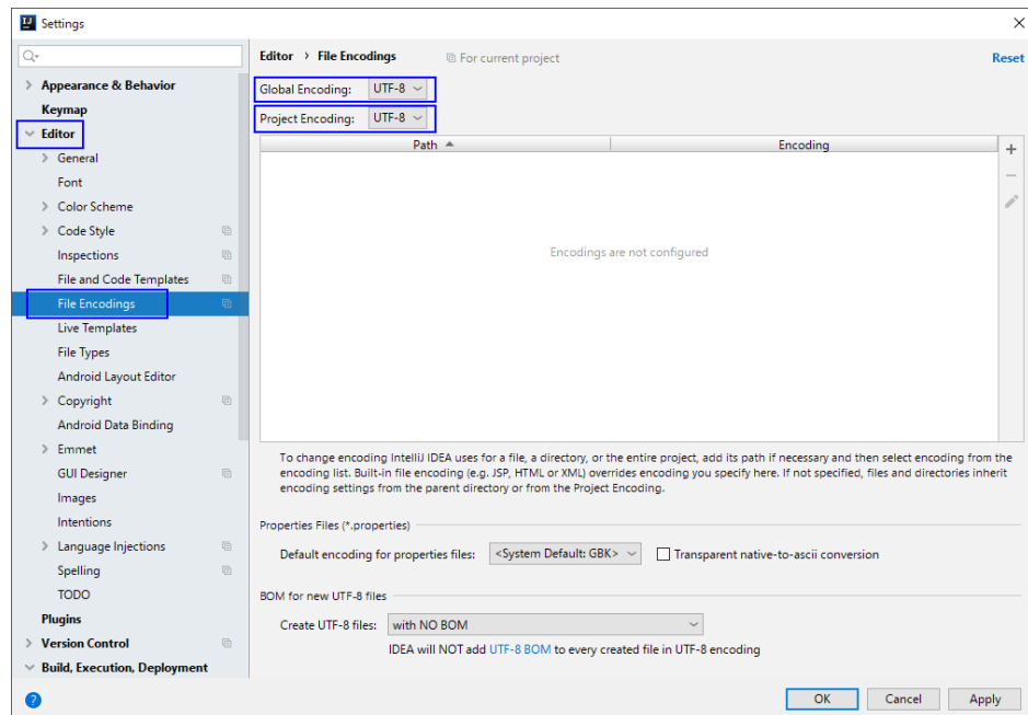
Figure 9-16 File Encodings
