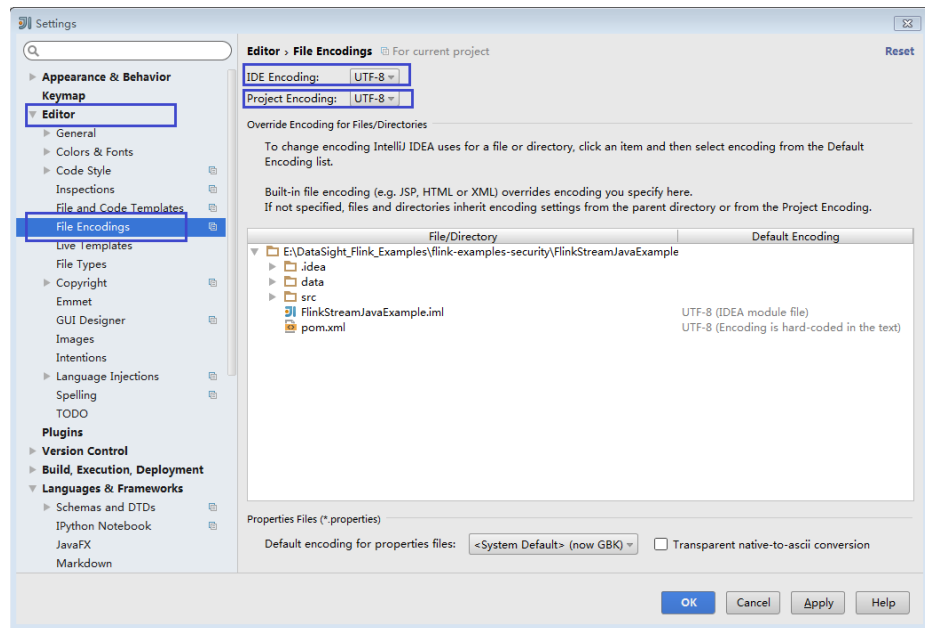
Figure 7-29 Settings
