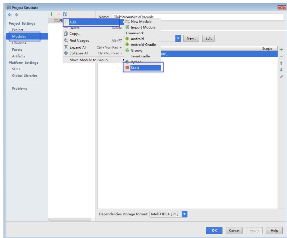
Figure 8-23 Selecting Scala
