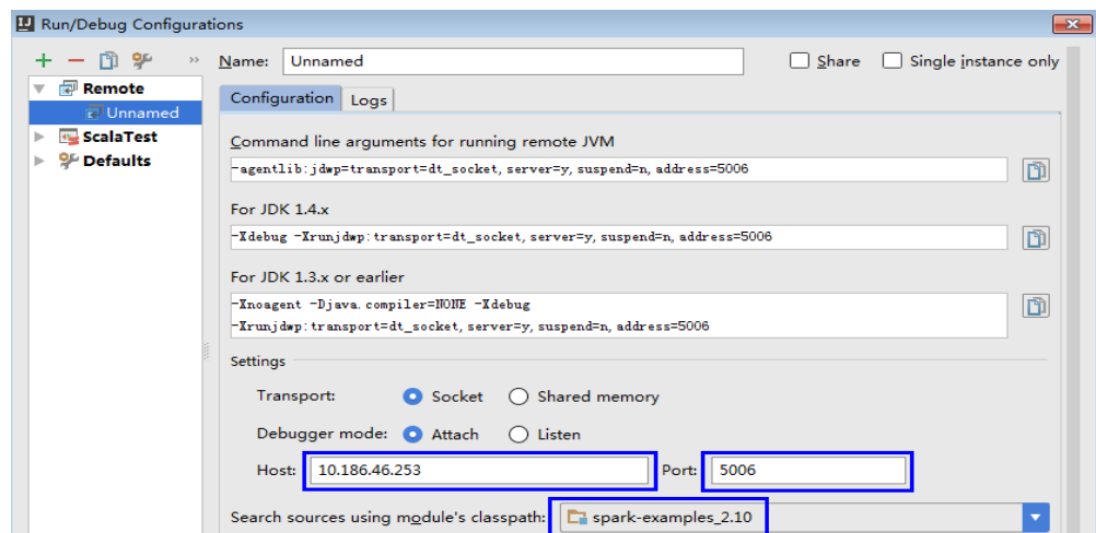
Figure 27-46 Configuring parameters
