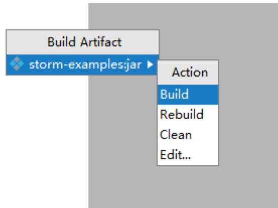
Figure 30-16 Build
