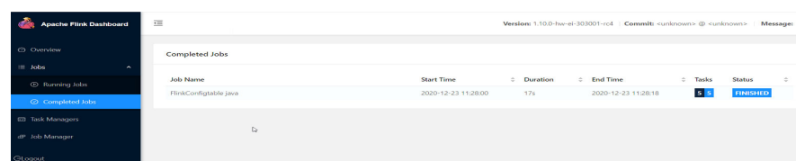
Figure 7-51 completed job
