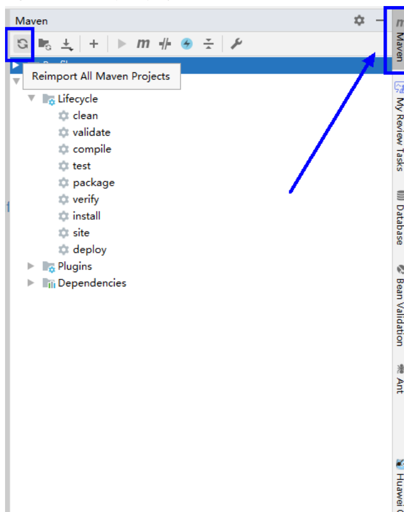
Figure 9-17 reimport projects
