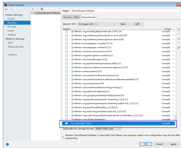
Figure 27-30 Successful configuration
