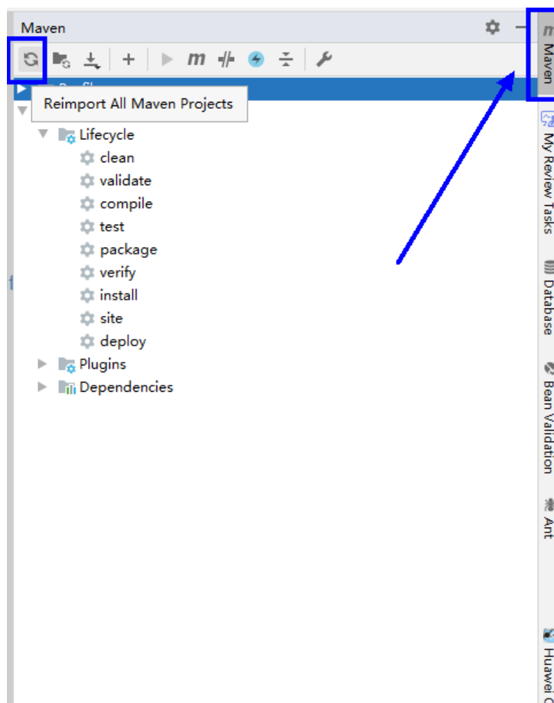
Figure 10-17 reimport projects
