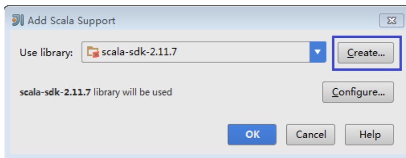
Figure 7-24 Create...
