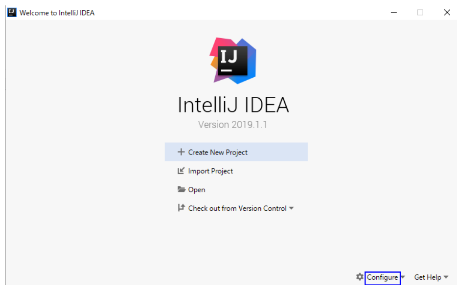
Figure 9-2 Quick Start
