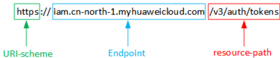
Figure 3-2 Example URI
