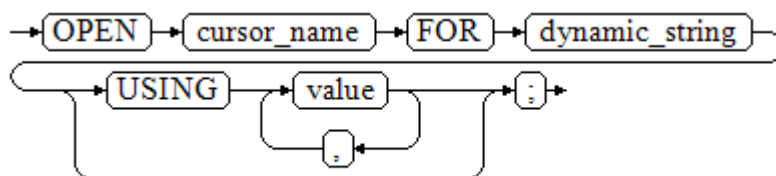
图 2-12 open_for::=
