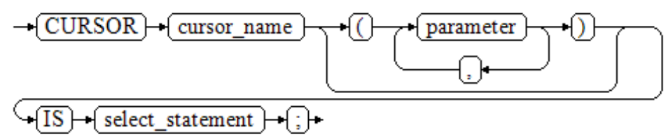
图 2-41 static_cursor_define::=
