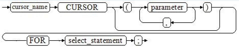
图 2-42 static_cursor_define::=
