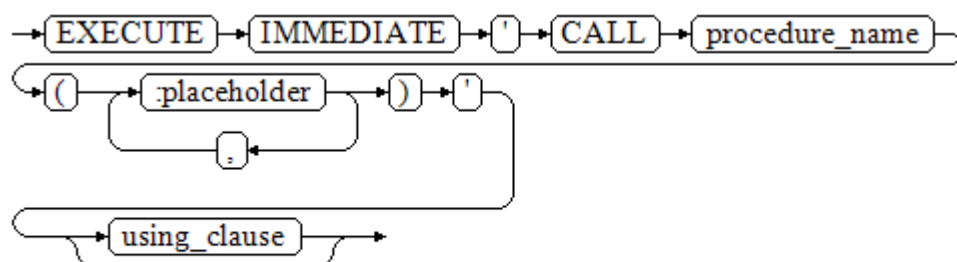
图 2-15 call_procedure::=
