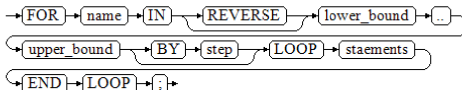
图 2-29 for_loop ::=
