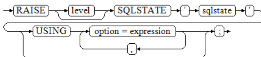
图 2-53 raise_sqlstate::=
