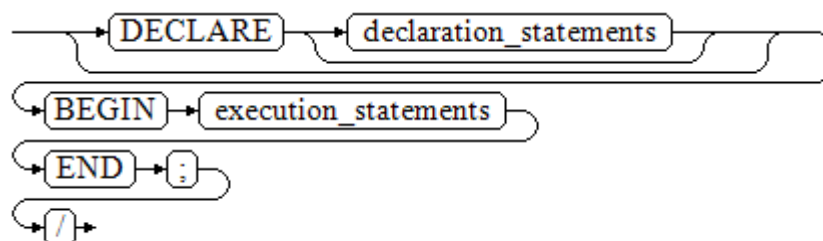
图 10-1 anonymous_block::=
