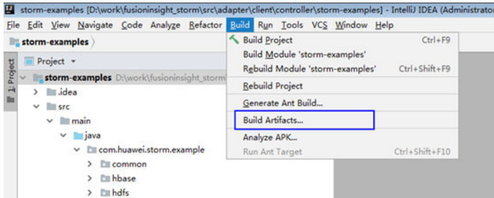
图 30-17 Build Artifacts
