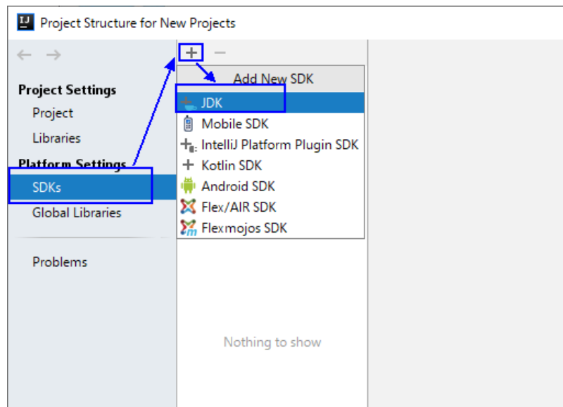
图 21-6 Project Structure for New Projects
