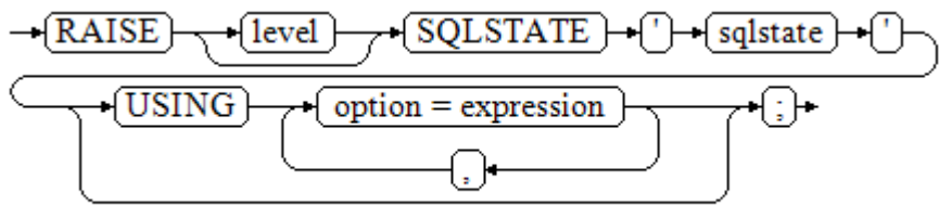
图 10-37 raise_sqlstate::=
