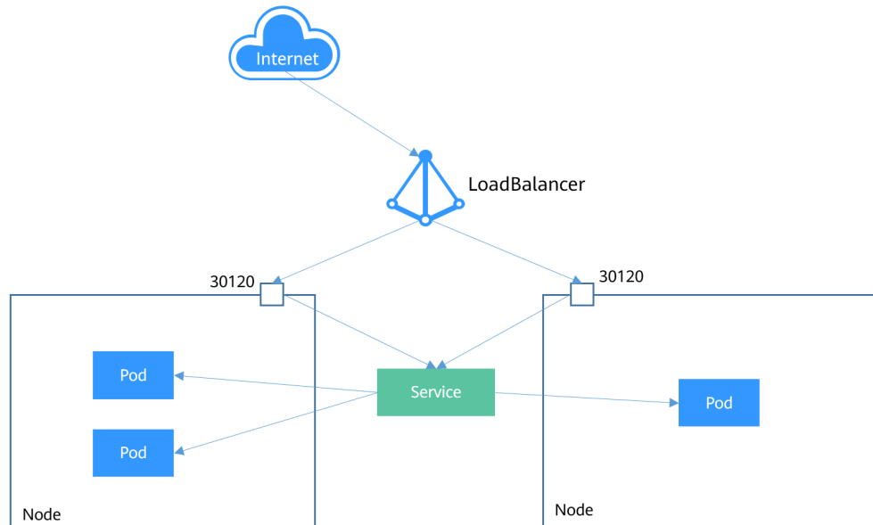
图 7-7 LoadBalancer Service
